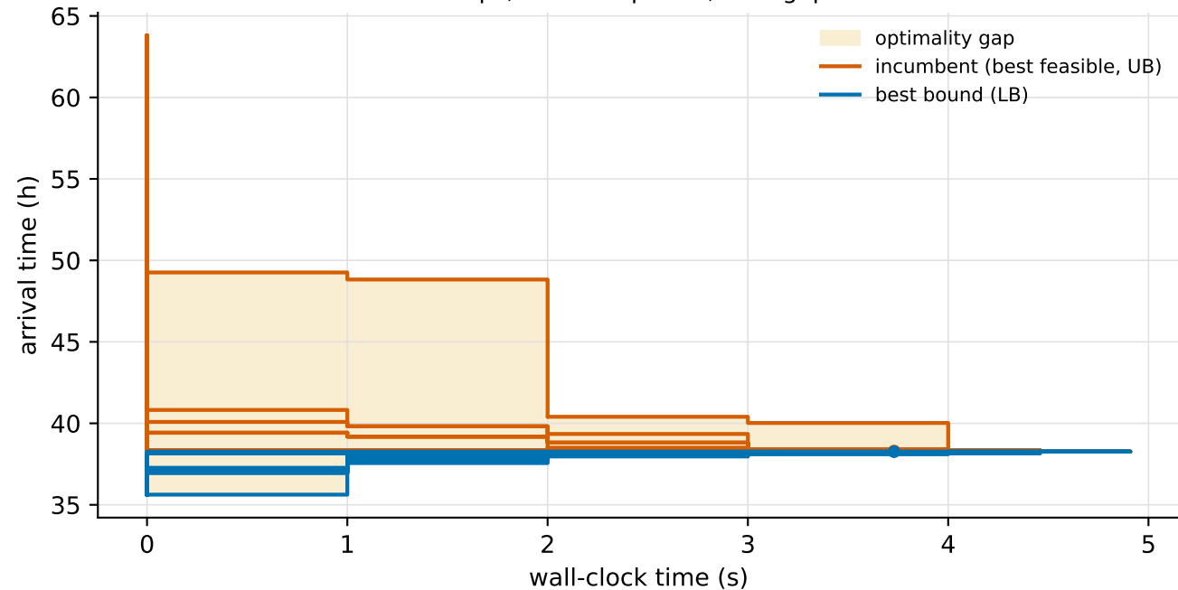
Oracle MIP bound evolution — RshortCfewTlarge_1 N=61 stops, status=optimal, final gap 0.12%
