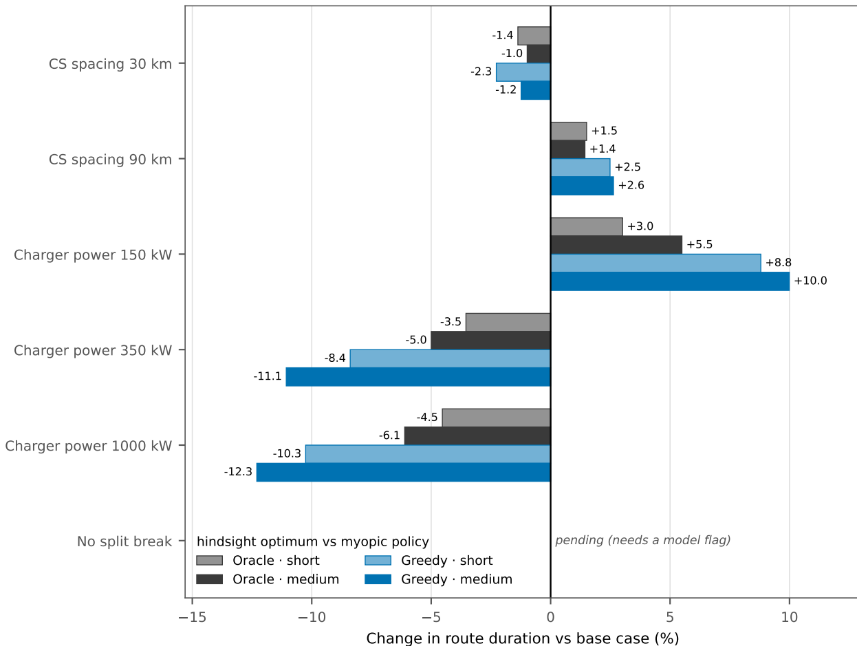
Sensitivity of route duration to charging infrastructure
