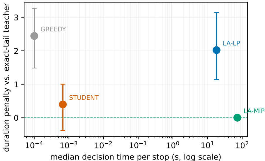
Solution quality against online decision latency
