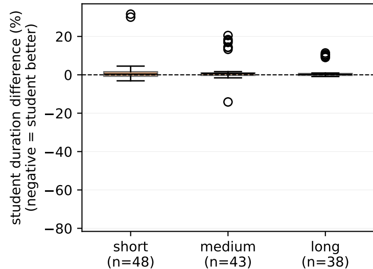
vs. exact-tail teacher
