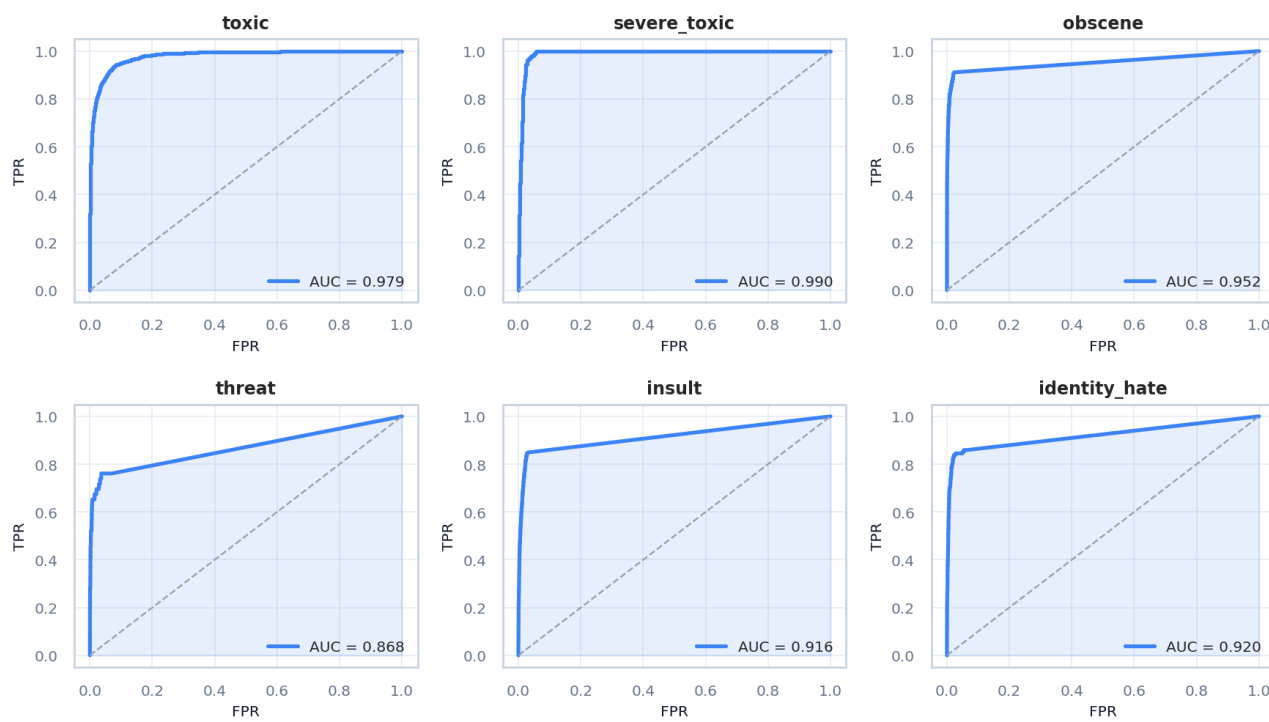
RNN — ROC Curves
