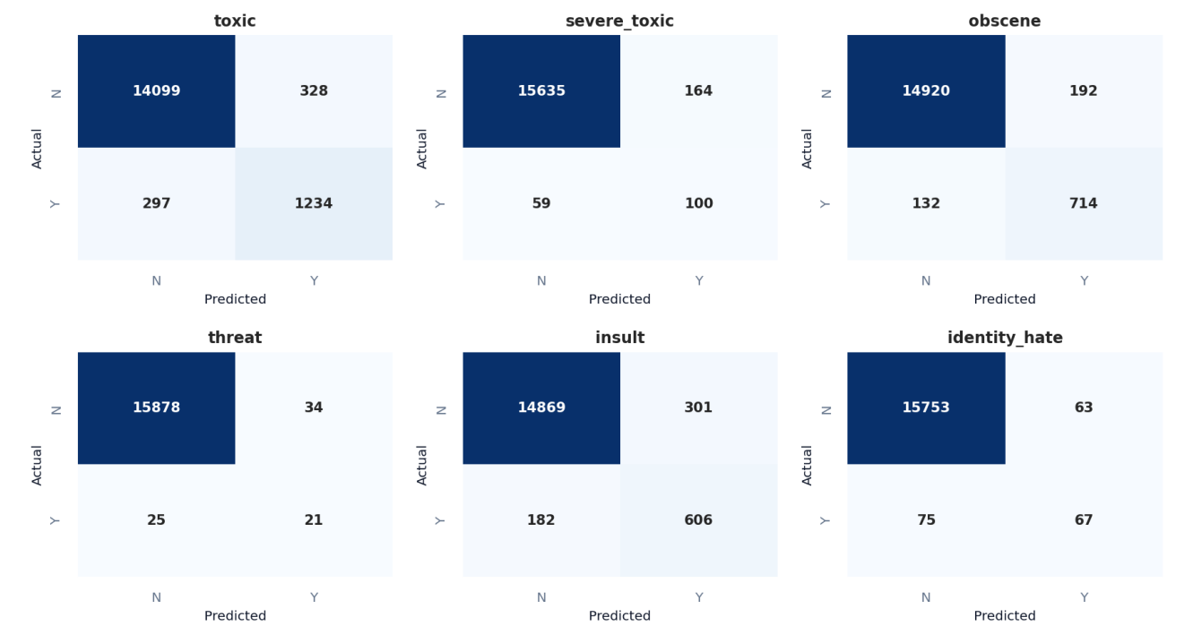
RNN — Confusion Matrices
