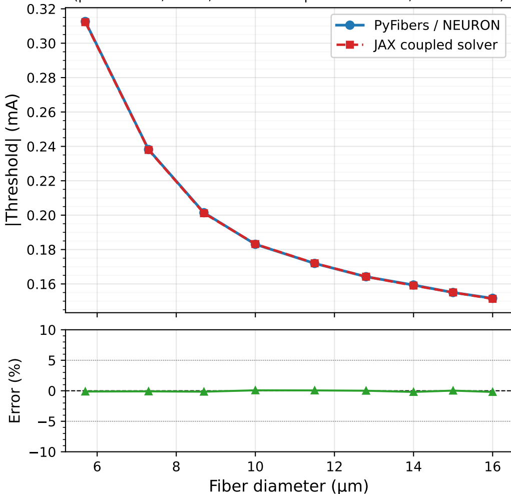
MRG activation threshold vs fiber diameter (point source, 1 mm, 0.1 ms monophasic cathodic, N=21 nodes)
