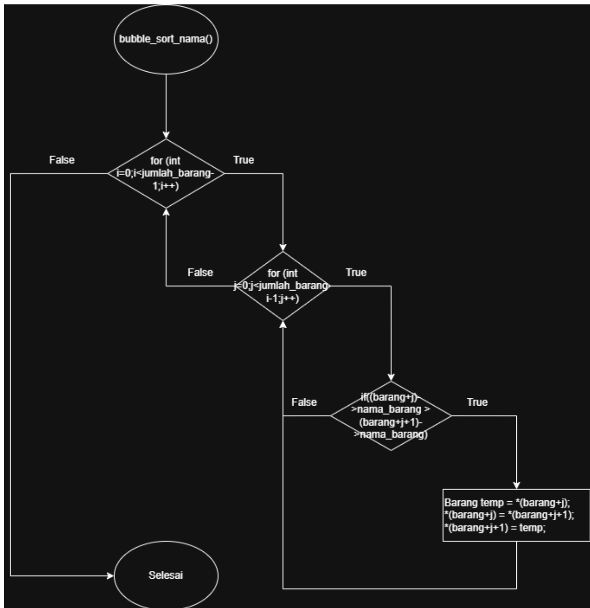
Gambar 1.10 Flowchart
