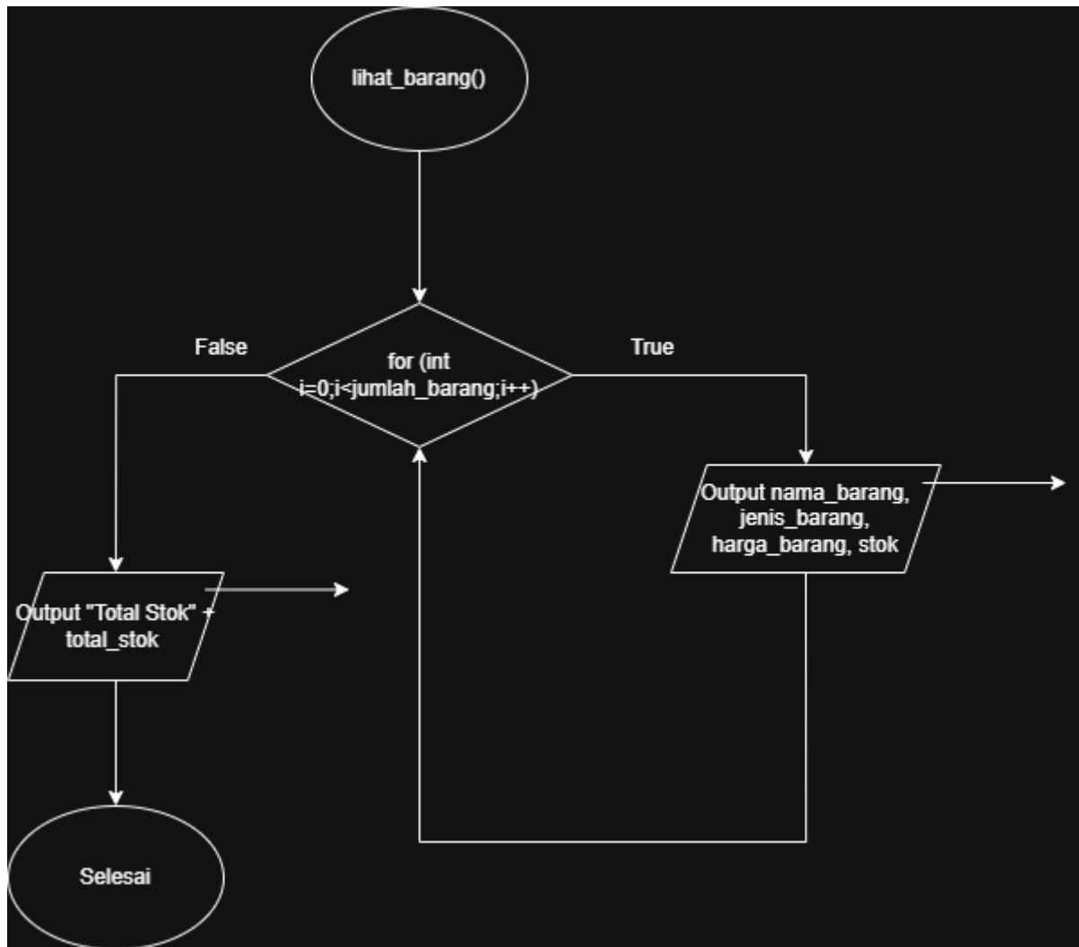
Gambar 1.7 Flowchart
