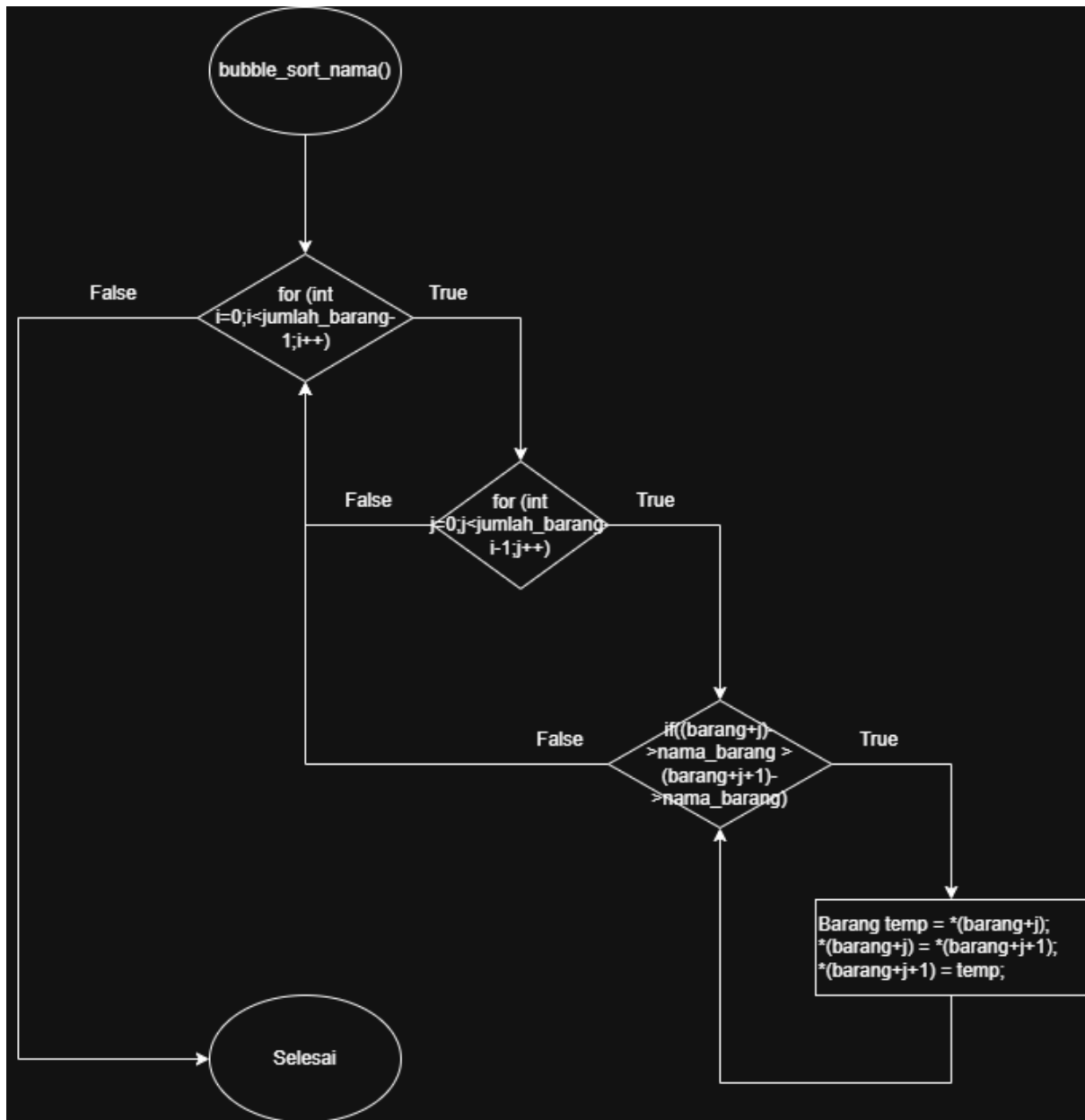
Gambar 1.10 Flowchart
