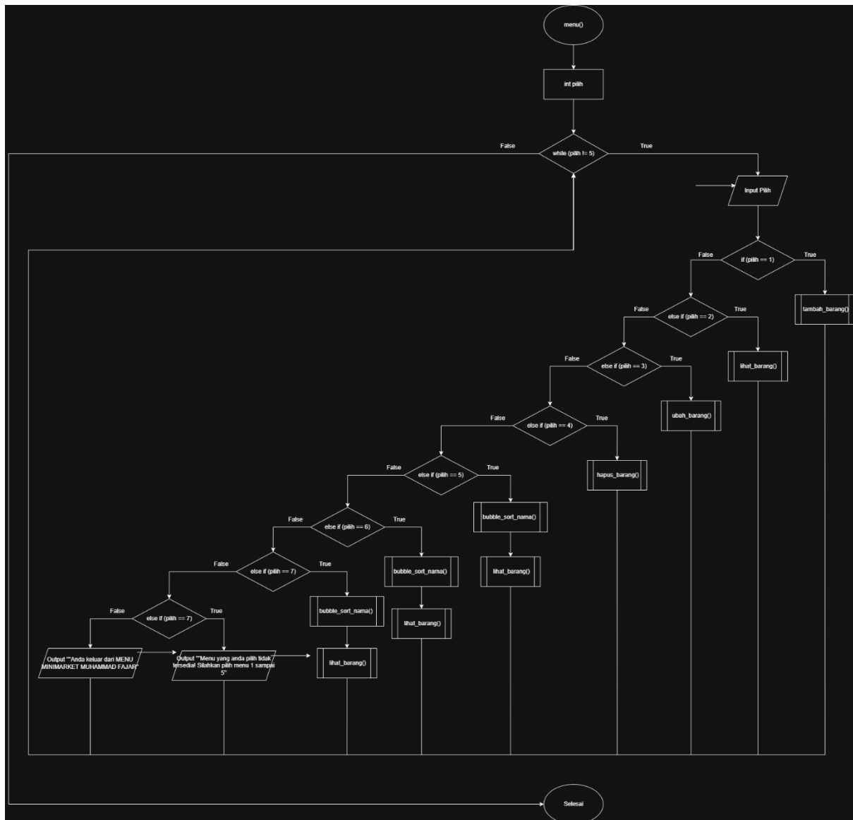
Gambar 1.5 Flowchart
