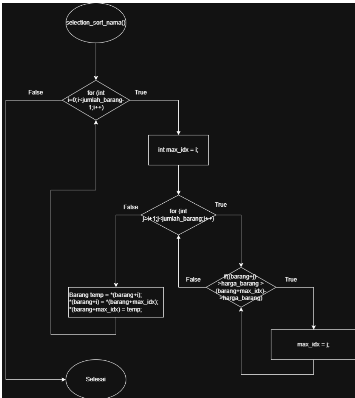
Gambar 1.11 Flowchart
