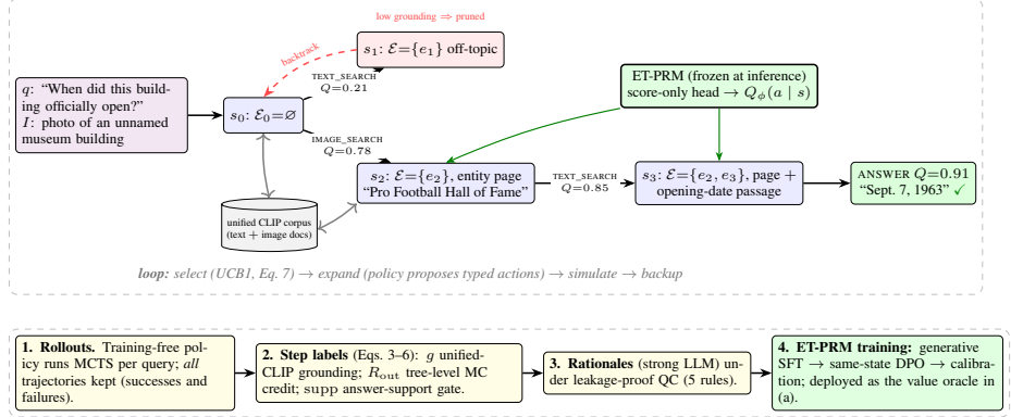
Figure 2: EvidenceTree overview. (a) The search tree lives in the retrieval action space : every edge is a typed action executed against the benchmark-provided corpus (one unified CLIP index for text and image documents), and every node is the resulting evidence state. The example illustrates the intended cross-modal plan on an entity question (the Q values are illustrative, not measured): a guessed \text{TEXT\_SEARCH} retrieves off-topic evidence and is pruned by its low PRM value ( Q=0.21 ); \text{IMAGE\_SEARCH} disambiguates the entity ( Q=0.78 ); a follow-up \text{TEXT\_SEARCH} on the evidence-established name fetches the asked attribute ( Q=0.85 ); the \text{ANSWER} edge closes the trajectory. UCB1 selection (Eq. 7) uses the PRM value as the only quality signal, so low- Q branches are abandoned — backtracking is a first-class operation. (b) The PRM is trained on ETBench-Open: MCTS rollouts are labeled per step with dual-source rewards and an answer-support gate, paired with QC-filtered rationales, and distilled into ET-PRM by generative SFT, same-state preference optimization, and calibration.
