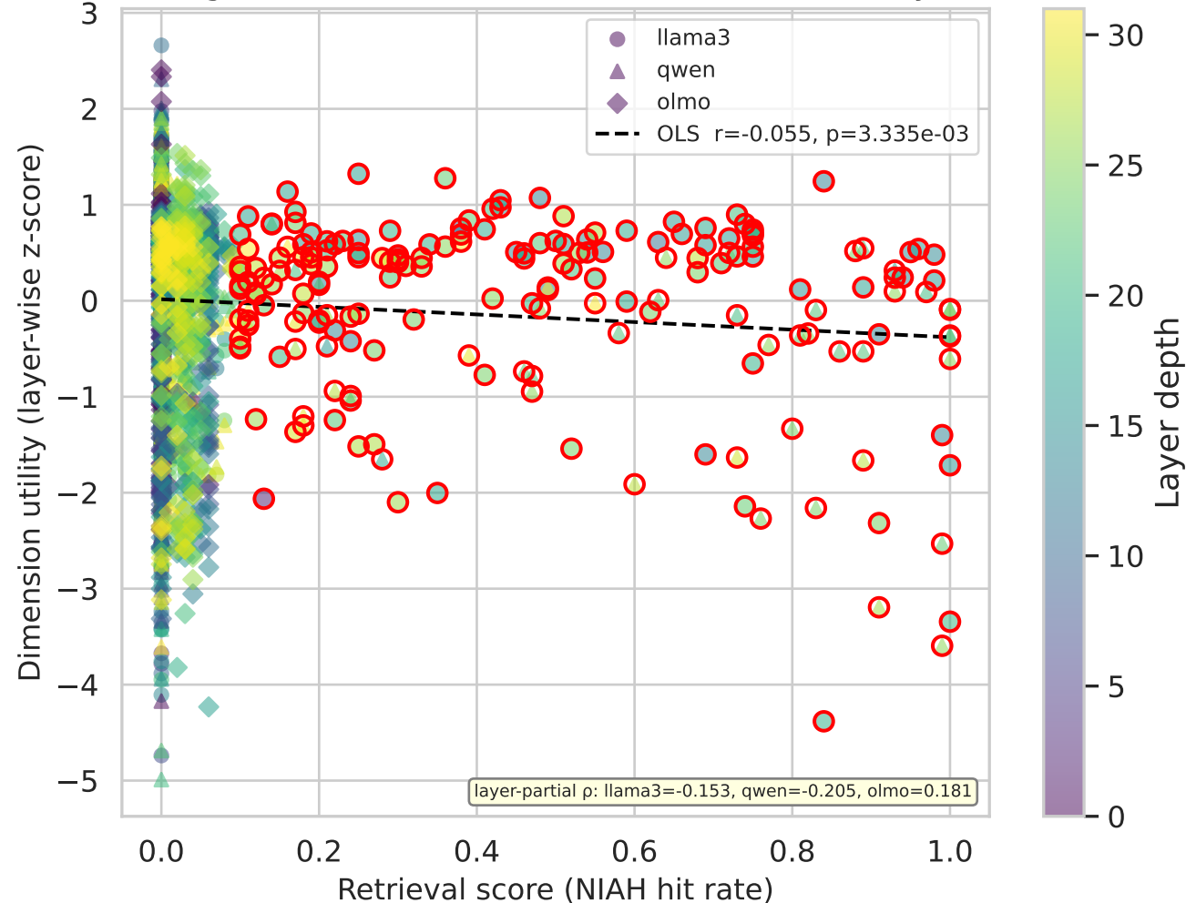
Figure 1 — Retrieval Score vs. Dimension Utility
