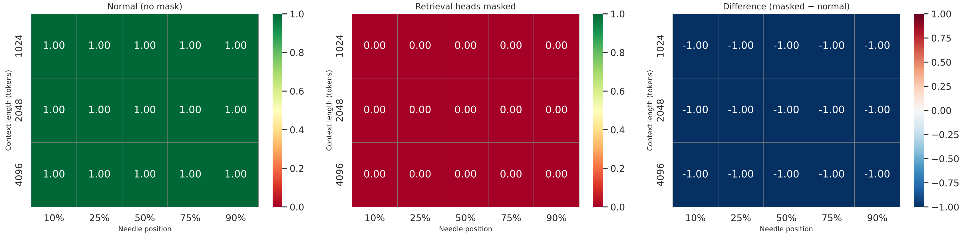
Figure 6 — NIAH Accuracy: Normal vs. Retrieval Heads Masked
