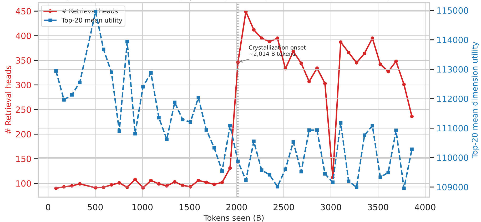
Figure 3 — OLMo-2 Training Dynamics
