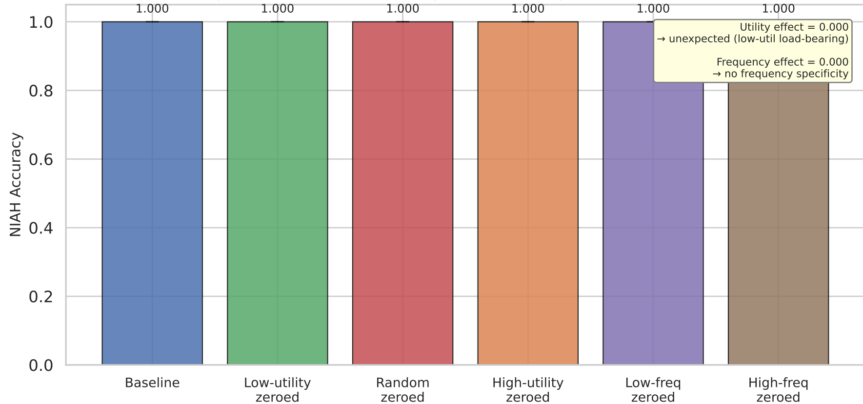
Figure 5 — Activation Patching: Dimension Importance for Retrieval
