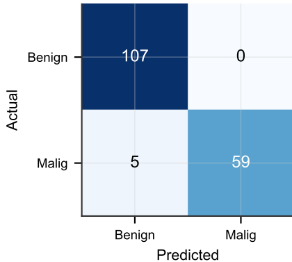
Random Forest
