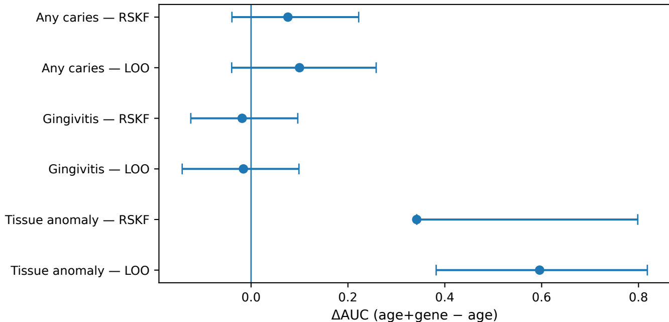
Model verification: \Delta AUC with 95% CI (Primary)
