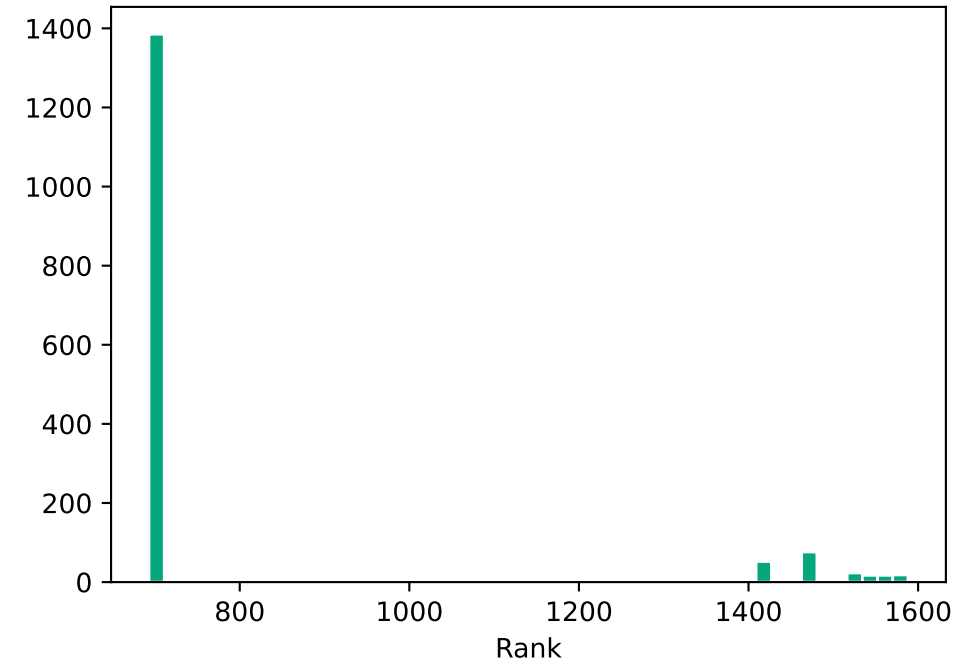
Rank-transformed skew=2.3
