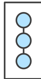
Commit History
