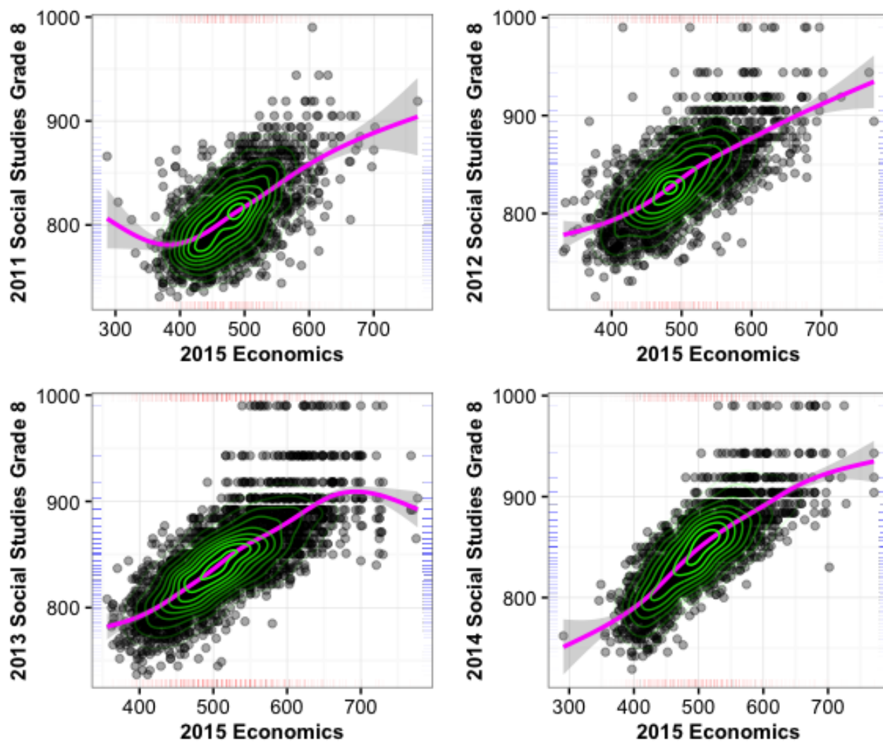
Fig. C.20: Conditional distribution(s) of current and prior scale scores: Economics.
