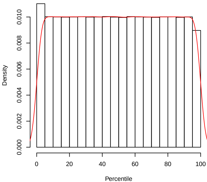
Standard SGP
