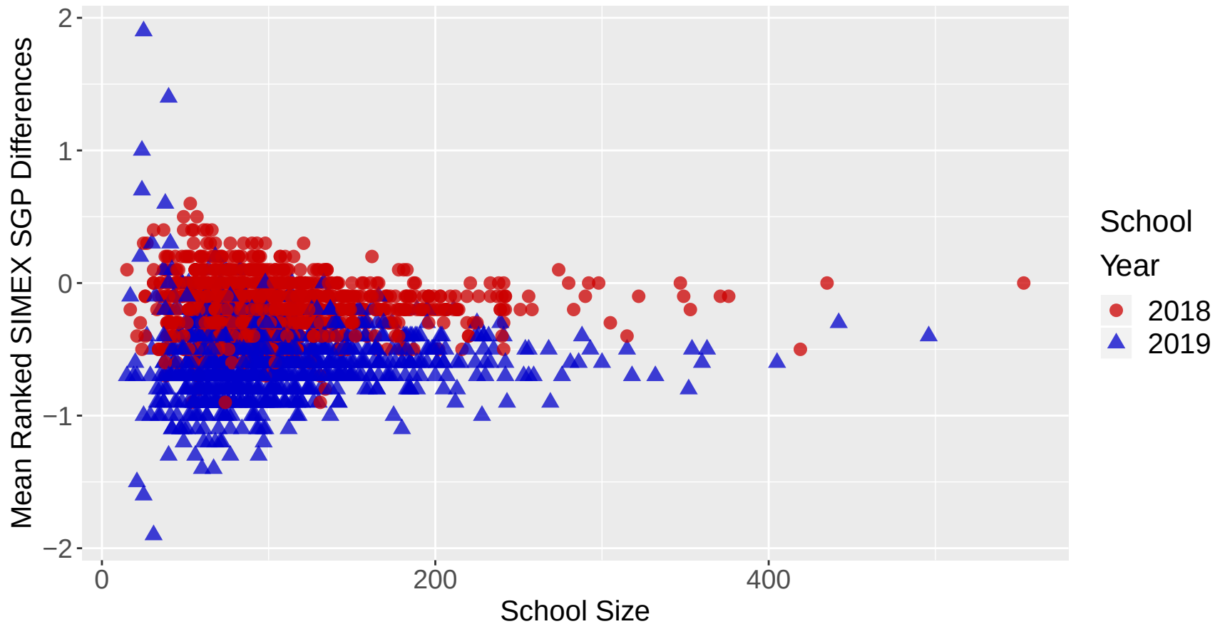
School Mean SGP Differences by School Size: Grade 5 Mathematics
