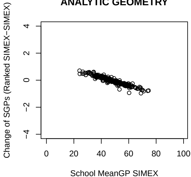
ANALYTIC GEOMETRY
