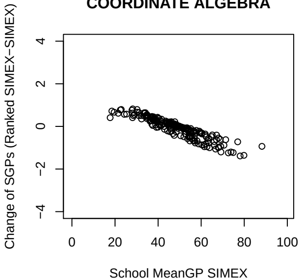
COORDINATE ALGEBRA
