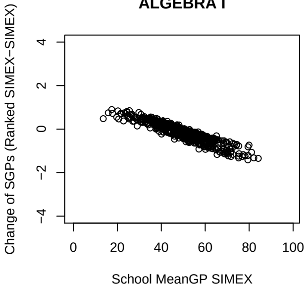
ALGEBRA I
