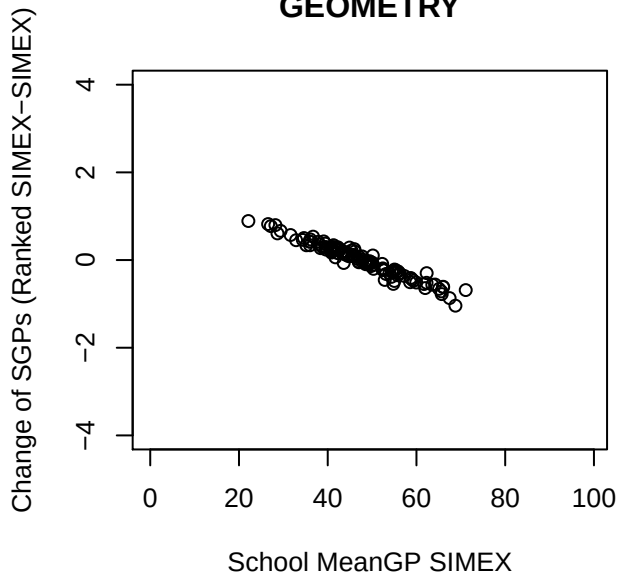
GEOMETRY
