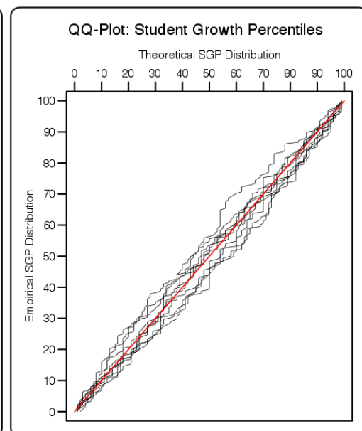
Figure 4: Goodness of Fit Plot for a 2016 SIMEX Corrected , Analytic Geometry Progression.
