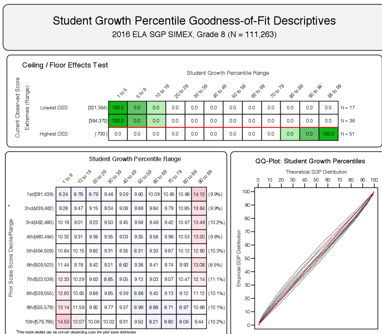
Figure 3: Goodness of Fit Plot for 2016 SIMEX Corrected , 8 th Grade ELA.
