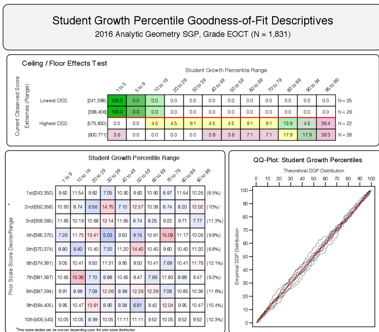
Figure 2: Goodness of Fit Plot for a 2016 Uncorrected Analytic Geometry Progression: Example of slight model mis-fit.
