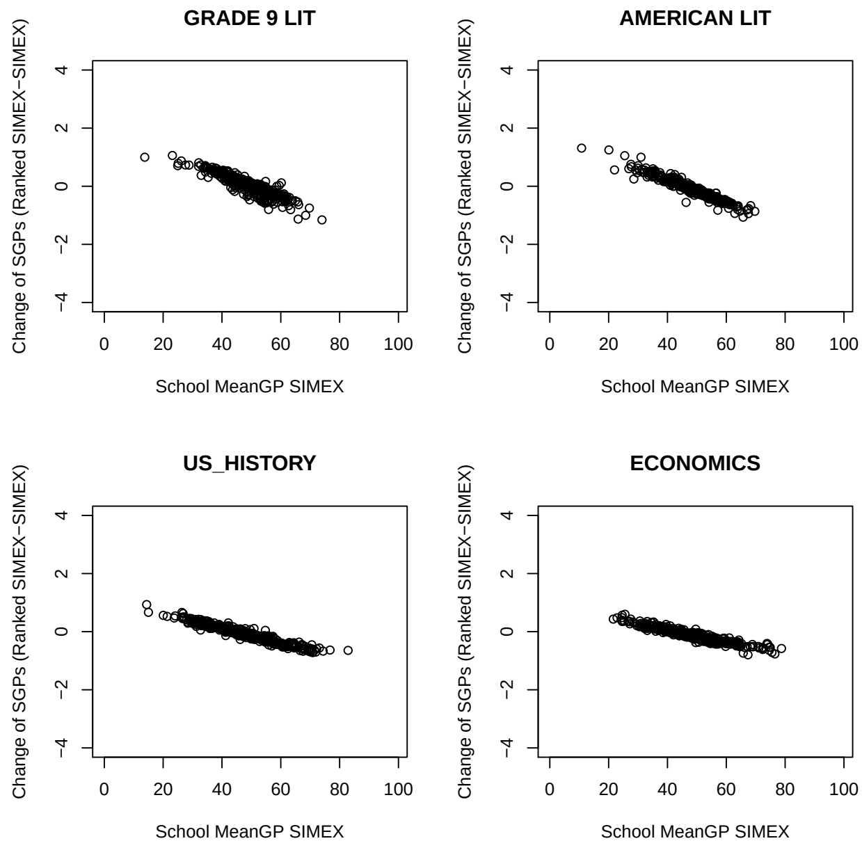
Figure 13: School MGP change (MGP Ranked SIMEX - MGP SIMEX) by EOC Subjects.
