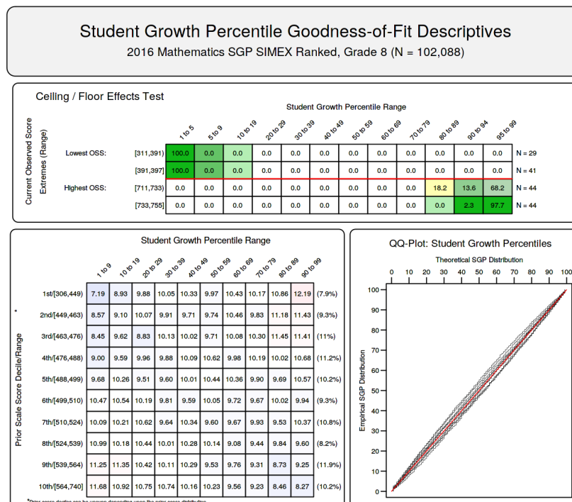
Figure 11: Goodness of Fit Plot for 2016 Ranked SIMEX 8 th Grade Mathematics SGPs.
