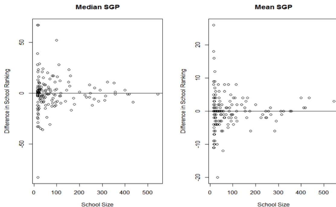
Figure 7: Difference in School Ranking in Different SIMEX Trials Plotted Against School Size for American Literature.
