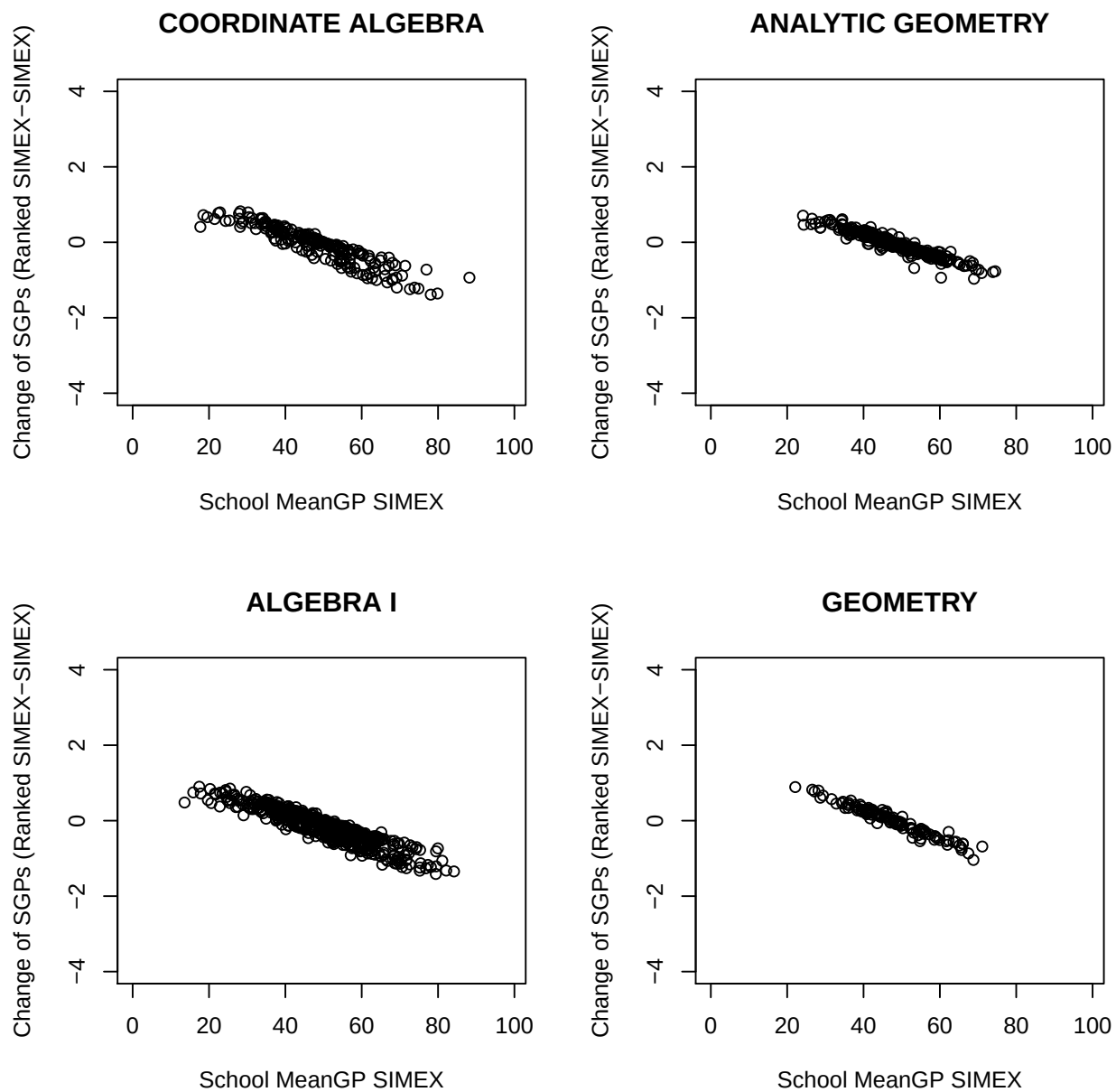
Figure 14: School MGP change (MGP Ranked SIMEX - MGP SIMEX) by EOC Subjects (Continued).
