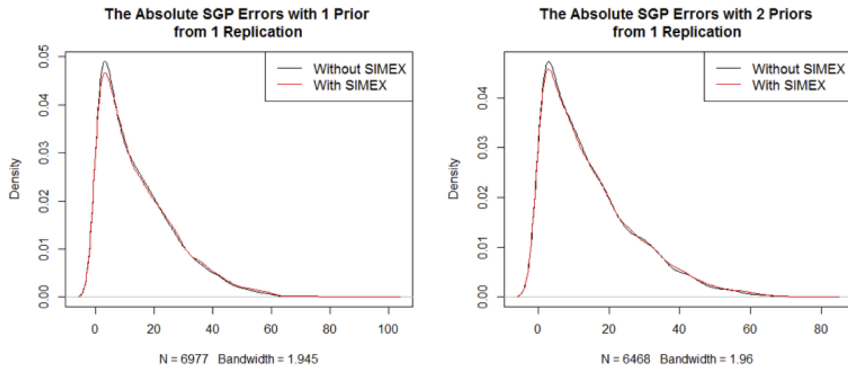
Figure 1: Absolute values of SGP Errors with 1 and 2 Priors Used.
