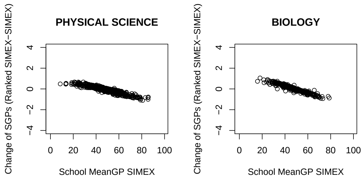
Figure 15: School MGP change (MGP Ranked SIMEX - MGP SIMEX) by EOC Subjects (Continued).
