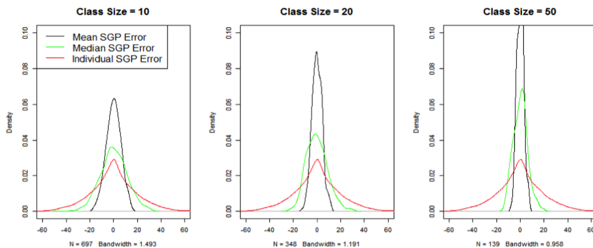
Figure 5: Errors of Aggregated and Individual SGPs of Grade 4.
