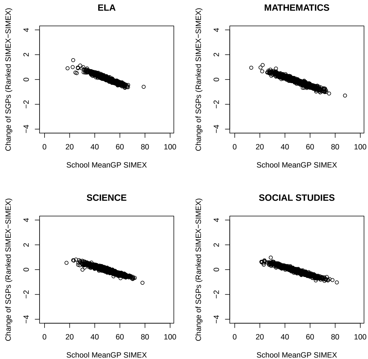
Figure 12: School MGP change (MGP Ranked SIMEX - MGP SIMEX) by EOG Subjects.
