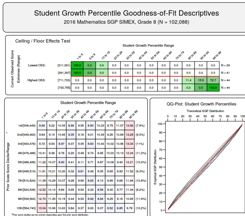
Figure 10: Goodness of Fit Plot for 2016 SIMEX 8 th Grade Mathematics SGPs.
