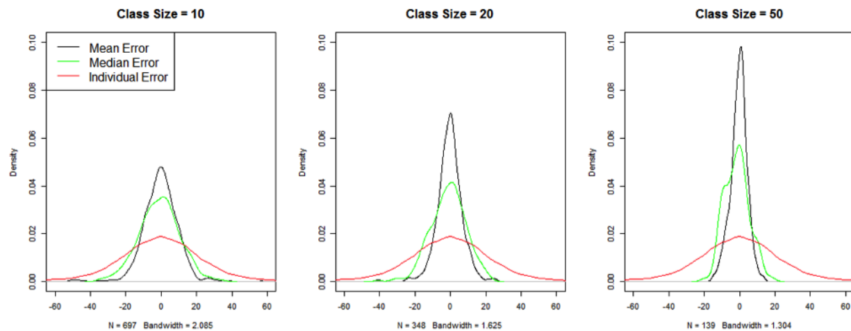
Figure 4: Errors of Aggregated and Individual Scale Scores of Grade 3.
