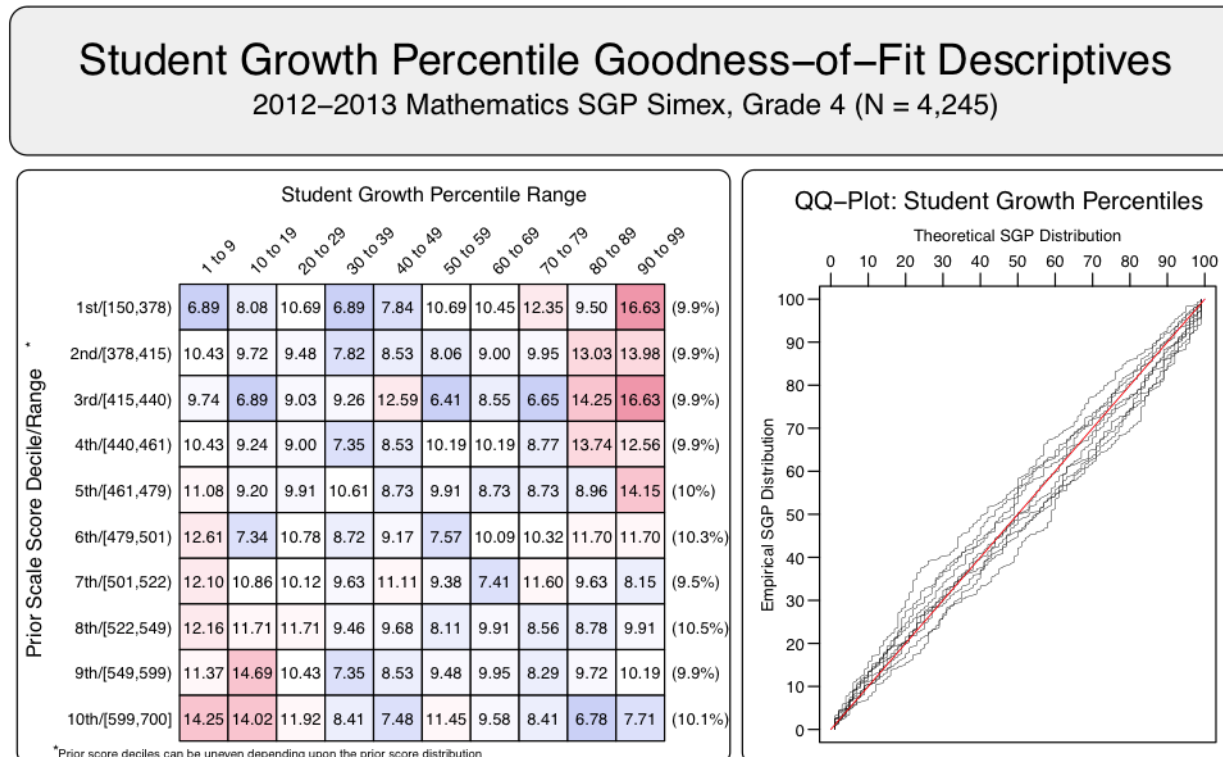
Figure 3: Goodness of Fit plot for SIMEX SGPs obtained from one 4 th grade simulation.
