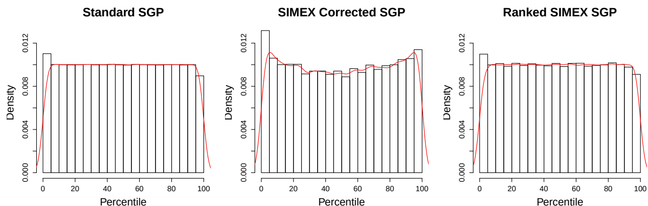
Figure 8: Comparison of the Uniformity of Distributions for 8 th Grade Mathematics Estimates.
