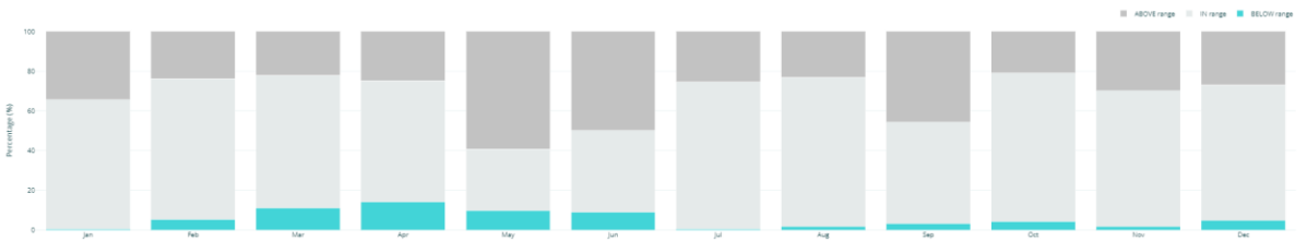
Cloud coverage
