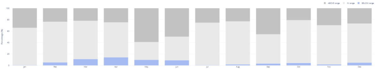
Cloud coverage
