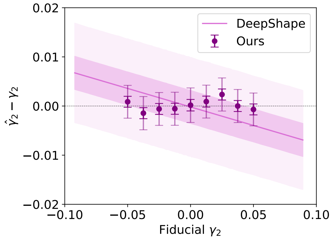
Shear Estimation with Error Bars (Ngal=10000)
