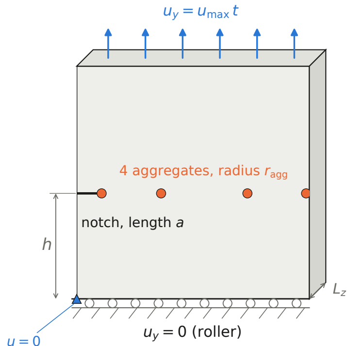
(a) geometry and loading
