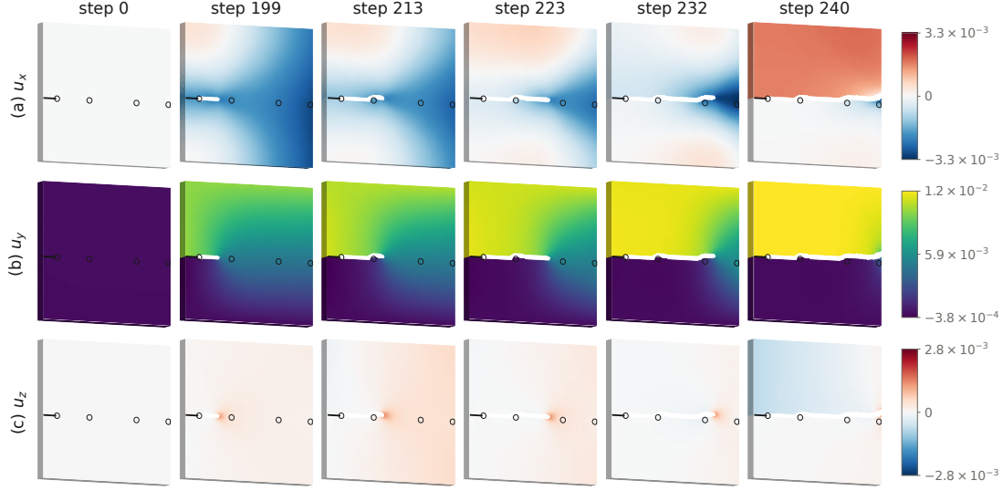
Figure 5: Evolution of the three displacement components for the realization of Figure 2(a,b), rendered on the three-dimensional specimen in the same view as Figure 3. Each row is one component ( u_x , u_y , u_z ) and each column one load step, with the steps chosen so that the crack tip advances by roughly equal increments between columns. Within a row the color scale is common to all steps, so the columns are directly comparable; between rows it is not, since the three components differ by more than an order of magnitude. Aggregate outlines are overlaid in black. The thin white band that opens along the ligament marks the fully damaged elements, which are removed rather than interpolated through because the displacement is discontinuous across an open crack. The dominant response is the mode-I opening in u_y , in which the two halves of the specimen separate almost rigidly; u_x concentrates around the advancing crack tip, and u_z reflects the through-thickness Poisson contraction.
