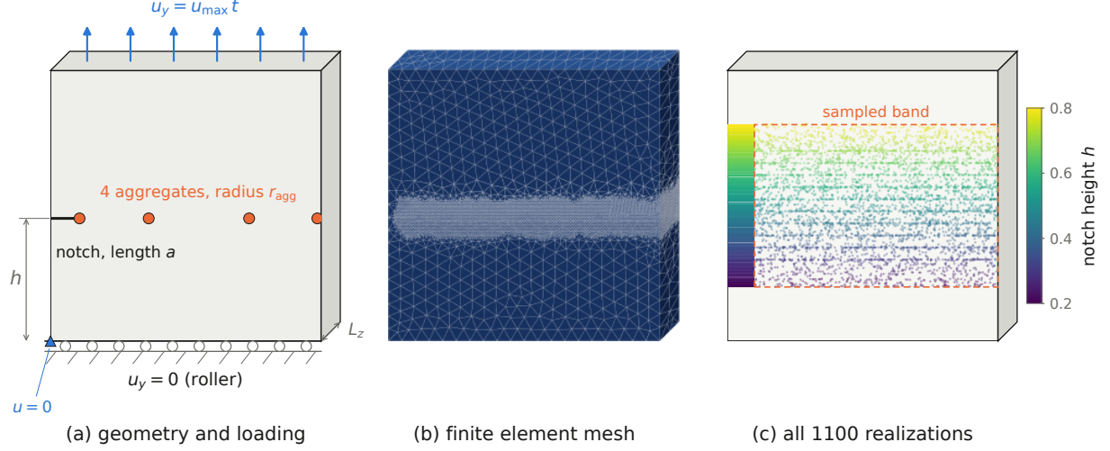
Figure 2: (a) Geometry and boundary condition setup for the concrete fracture simulations. A plate of dimensions 1.0 \times 1.0 \times 0.1 contains a pre-existing horizontal notch of length a at height h , together with four stiff aggregate inclusions centered on the ligament ahead of the notch tip. A monotonically increasing tensile displacement is applied on the top boundary. (b) Tetrahedral finite element mesh of a representative realization, shown in the same oblique view as (a); the refined band that follows the sampled notch height and the expected crack path is clearly visible, and the mesh is regenerated for every realization. (c) All 1100 realizations at once, on the same plate and in the same view: the 4400 aggregate centres, and on the left face the notch trace of every realization, both coloured by notch height. The dashed box is the region the inputs are drawn from, x_i \in [0.1, 1] and h \in [0.2, 0.8] ; the plate is drawn in full so the unsampled margins are visible.
