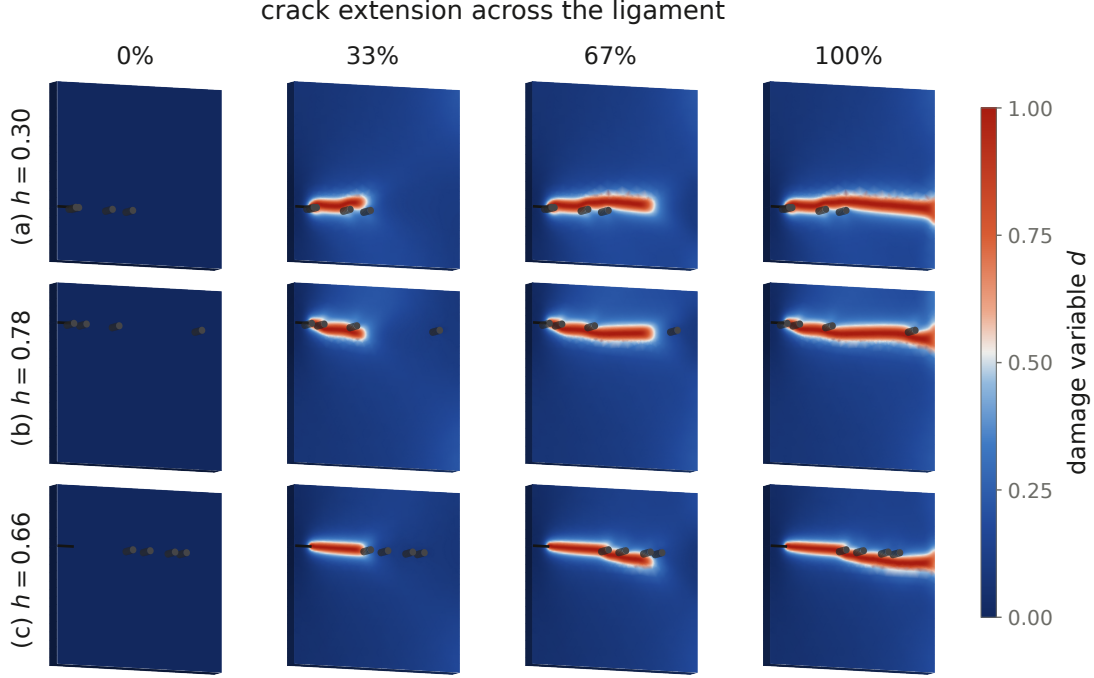
Figure 3: Damage evolution for three realizations (rows) with different aggregate arrangements under identical loading, rendered on the three-dimensional specimen. Columns correspond to equal fractions of the ligament crossed by the crack tip, selected separately for each realization because the fronts advance at different rates; the load step behind each column is therefore not the same across rows. The dark slit on the left face is the notch and the dark cylinders are the aggregate inclusions, which run through the full thickness. Depending on whether the aggregates lie on or off the ligament, the crack propagates straight through, deflects around an inclusion, or is temporarily arrested before resuming, demonstrating the range of fracture behaviors captured in the dataset.
