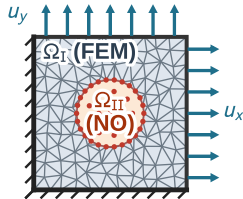
Case 3: Elastodynamic disk, u_x = u_y = 0.01
