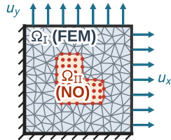
Case 4: Elastodynamic L-shape, u_x = u_y = 0.01
