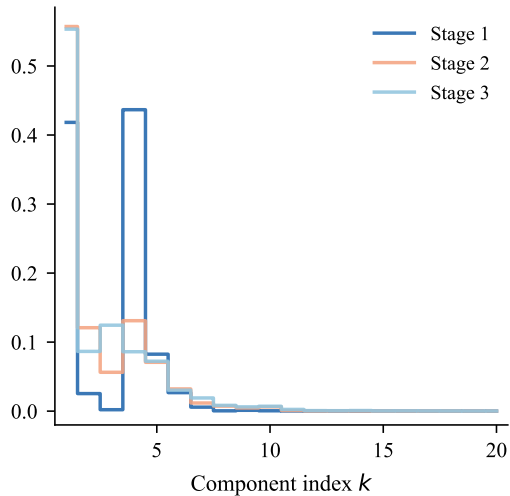
\rho_2 = 0.5, \rho_3 = 0.7 (Moderate dependence)
