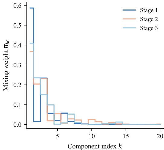
\rho_2 = \rho_3 = 0 (Independent DPs)
