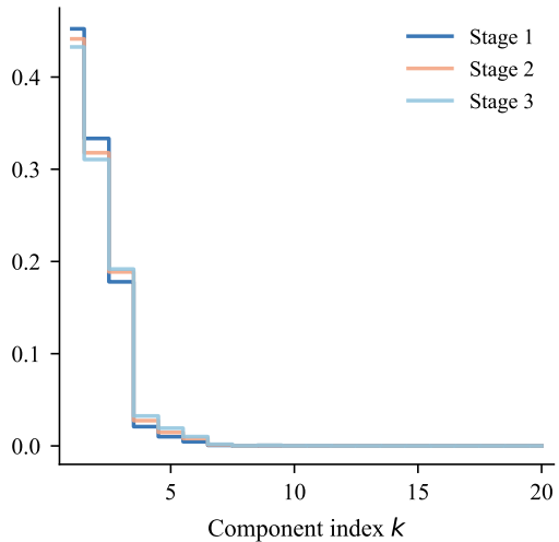
\rho_2 = 0.9, \rho_3 = 0.95 (Strong dependence)
