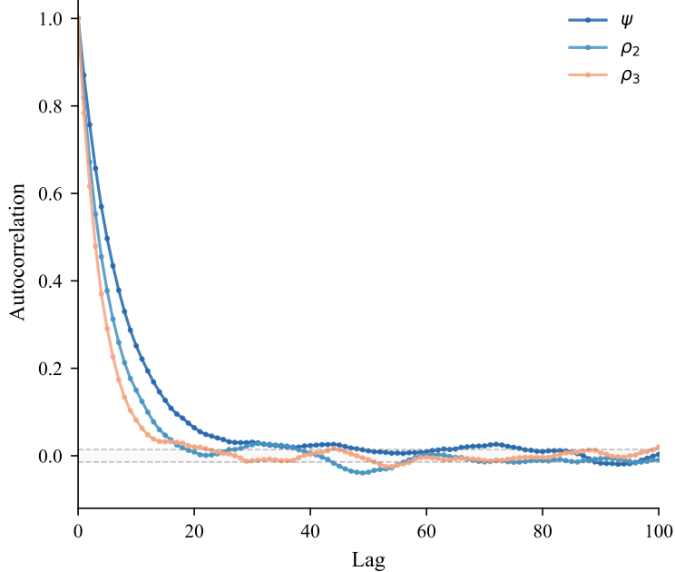
(a) ACF: \psi, \rho_2, \rho_3
