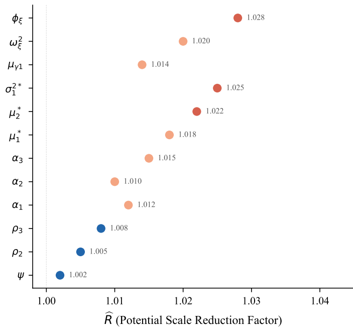
(c) Gelman-Rubin Convergence Diagnostic \hat{R}
