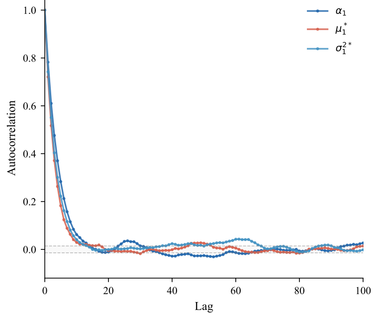
(b) ACF: \alpha_1, \mu_1^*, \sigma_1^{2*}
