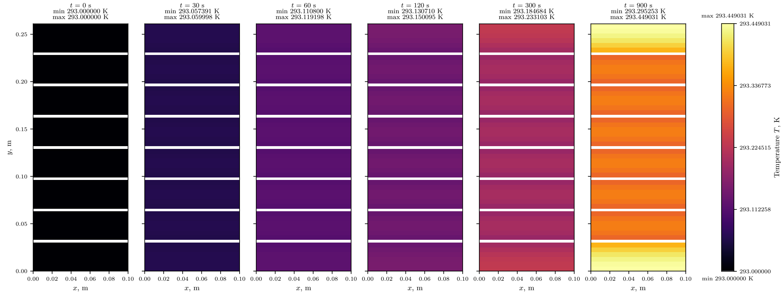
Module temperature on the mesh, 960 cells
