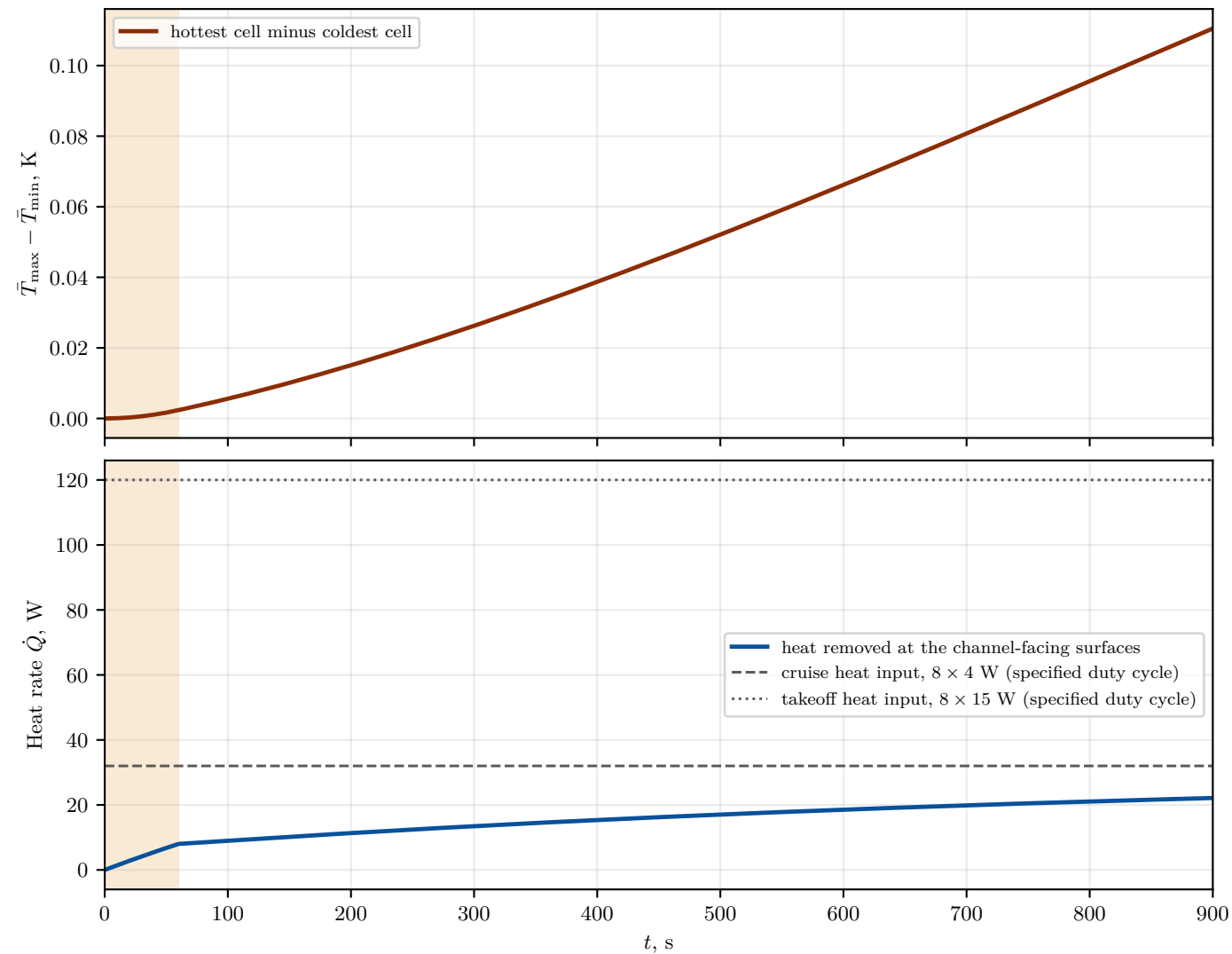
Pack uniformity across the eight cells (shaded band: takeoff power pulse)
