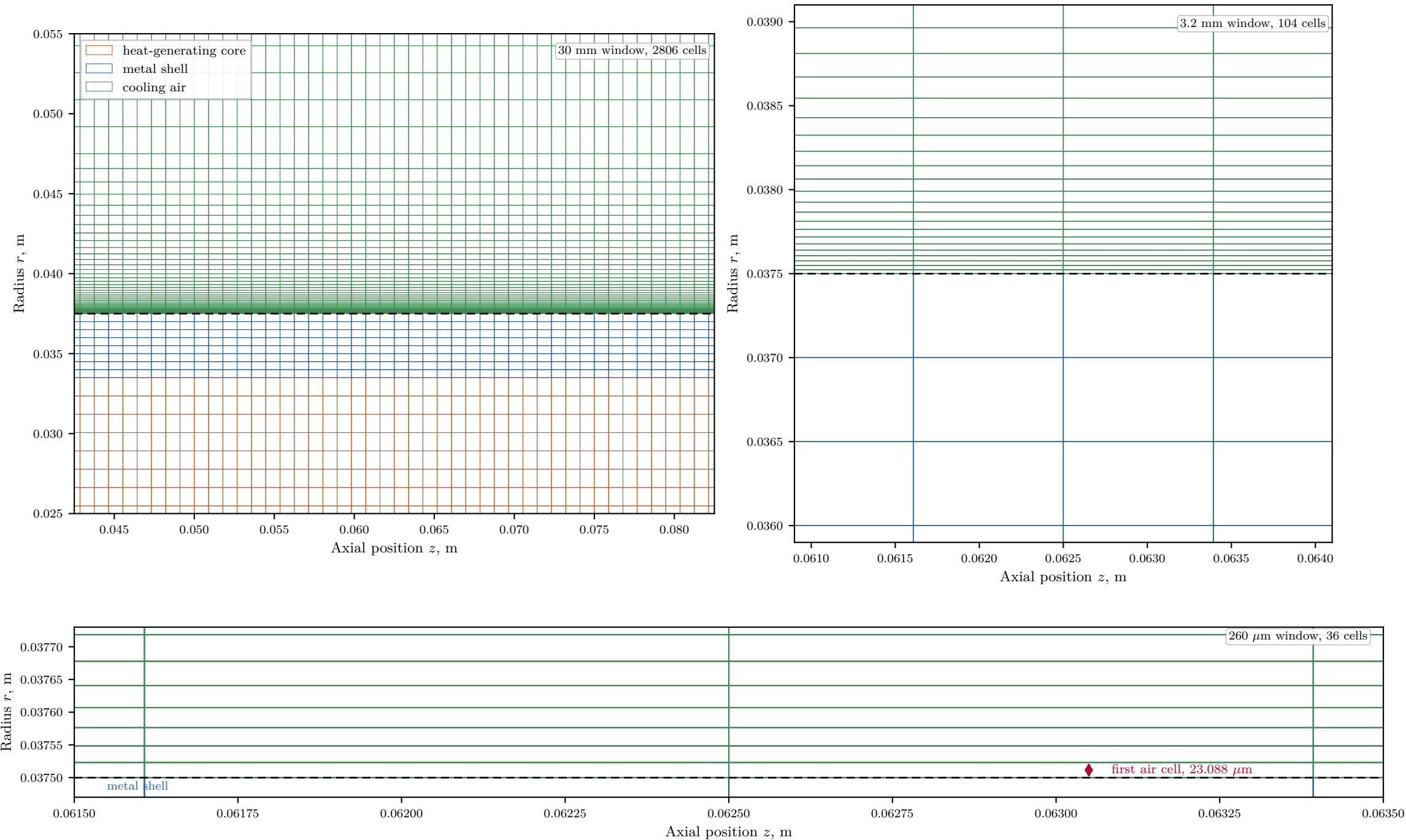
Computational mesh at the cooled surface, three zooms
