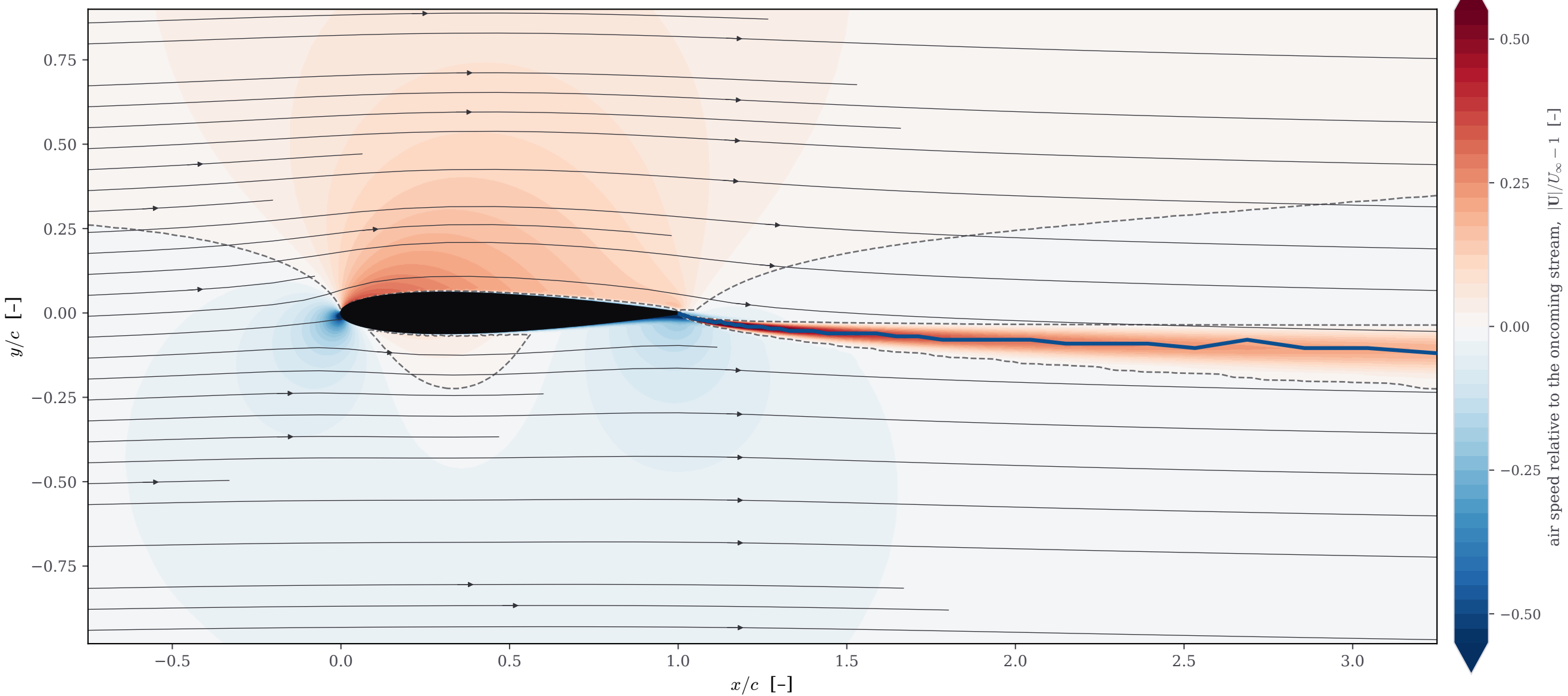
Speed relative to the oncoming stream, with the jet sheet traced and streamlines entering at equal spacing.
