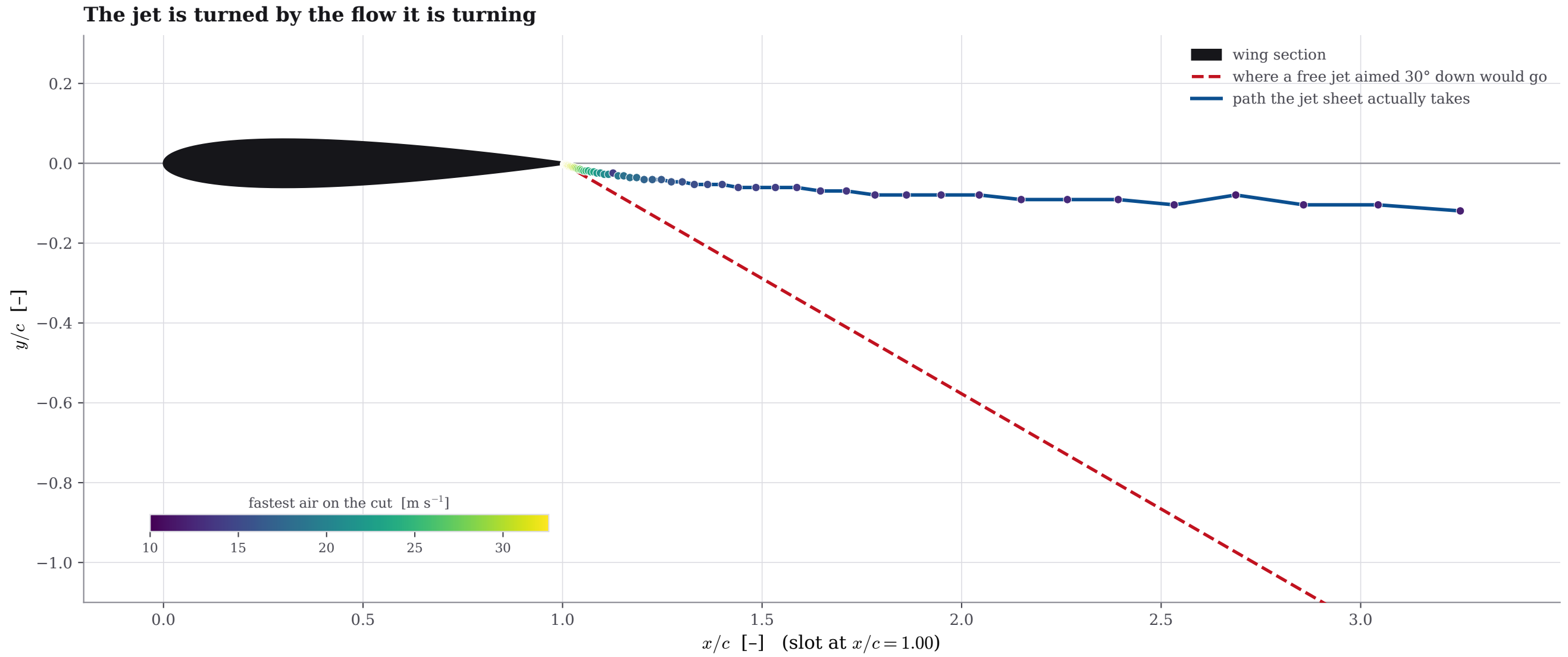
The ejected sheet leaves at thirty degrees and is turned by the oncoming flow; colour is peak speed.
