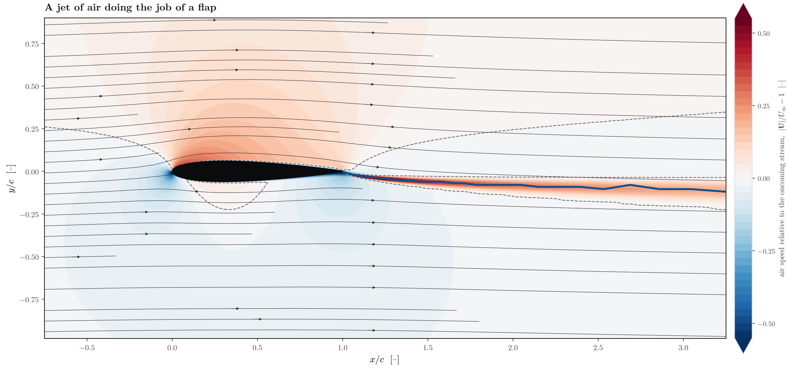
Speed relative to the oncoming stream, with the jet sheet traced and streamlines entering at equal spacing.
