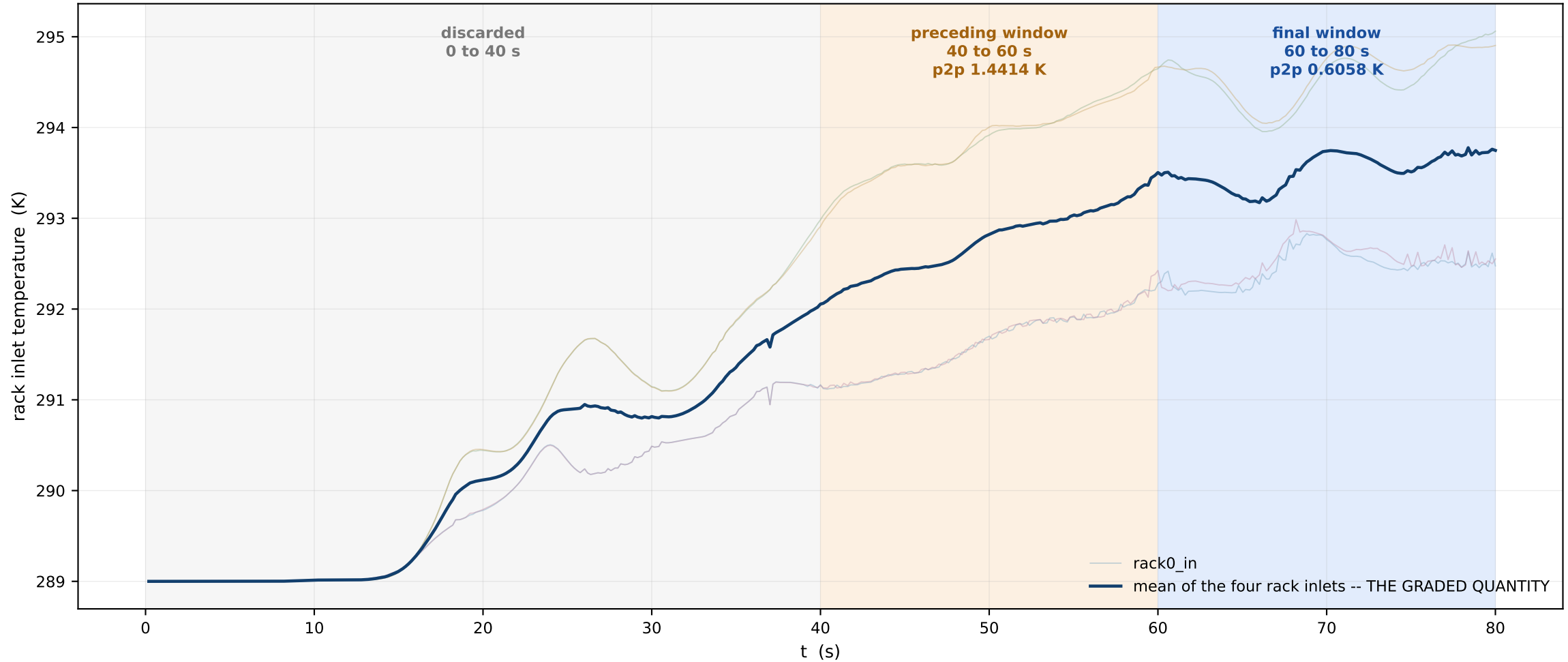
K2bU3R3 rack inlet temperature: the oscillation DAMPS in 3-D -- ratio 0.420 against a registered DAMPS threshold of 0.5 or below
