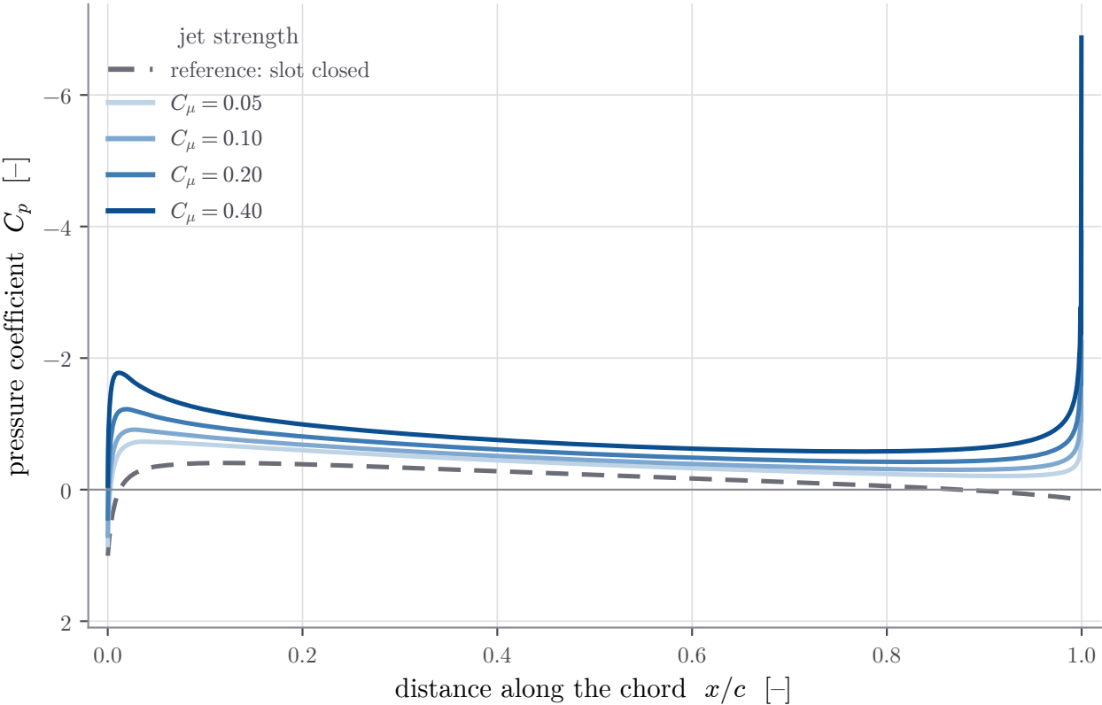
Upper (suction) surface, full scale
