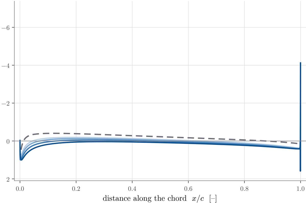
Lower (pressure) surface, full scale
