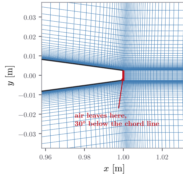
C. Trailing edge and the slot
