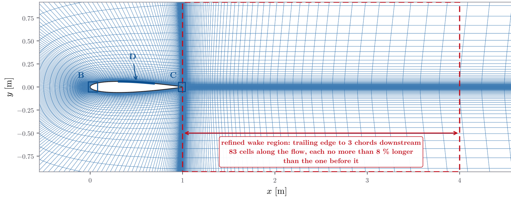
A. Around the wing and through the wake (the whole grid reaches 25 m in every direction)
