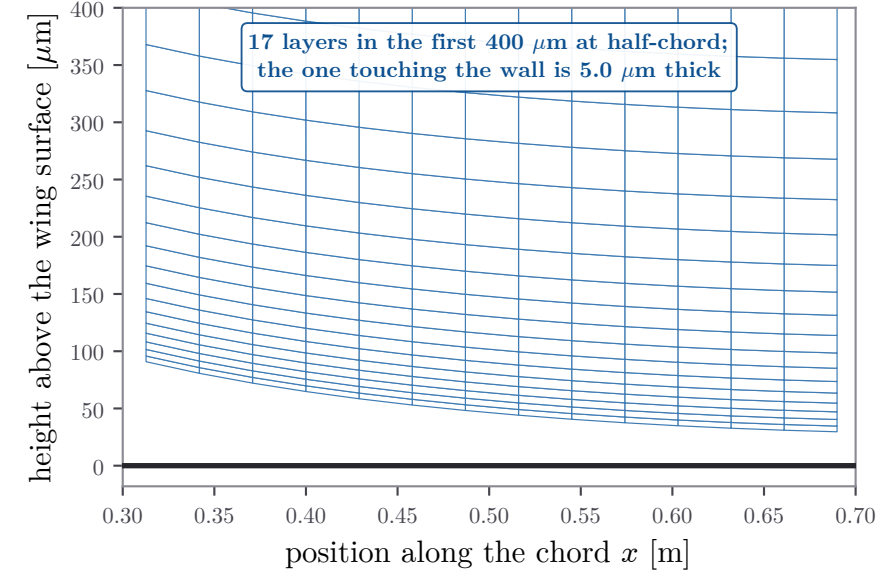
D. The layers packed against the wall (height measured up from the surface)
