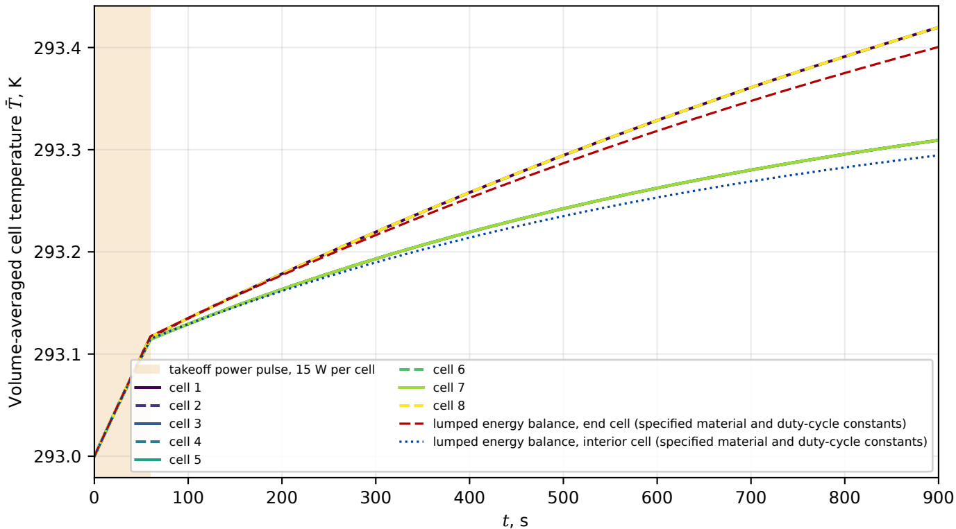
Cell temperature histories, volume-averaged over the 120 mesh cells of each cell Cells 1 and 8 coincide; cells 2-7 coincide (difference 0.000 \times 10^0 K)
