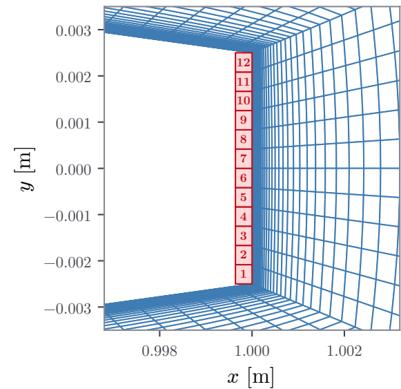
D. Cells across the slot: 12
