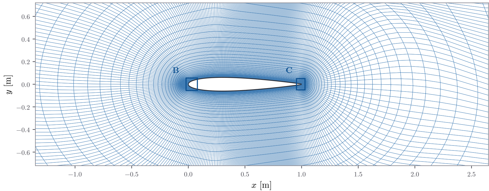
A. Around the wing (the whole grid reaches 26 m in every direction)
