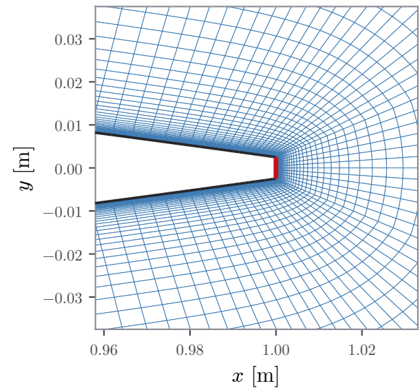
C. Trailing edge and the slot
