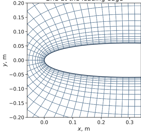
Grid at the leading edge
