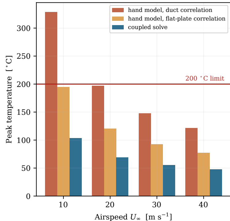
Hand model against the solve, at P = 305 \text{ W}
