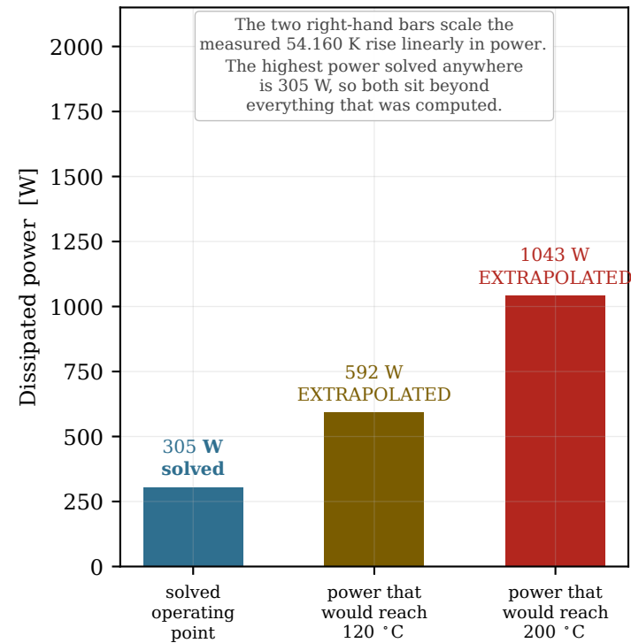
Power headroom implied at U_{\infty} = 20 \text{ m s}^{-1}
