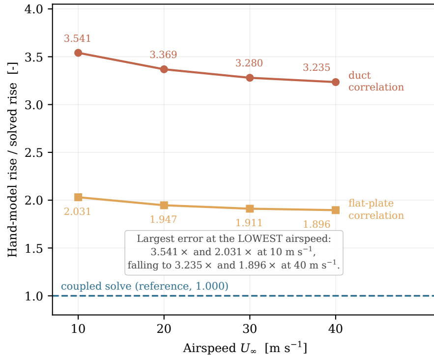
The hand model's overprediction SHRINKS as airspeed rises
