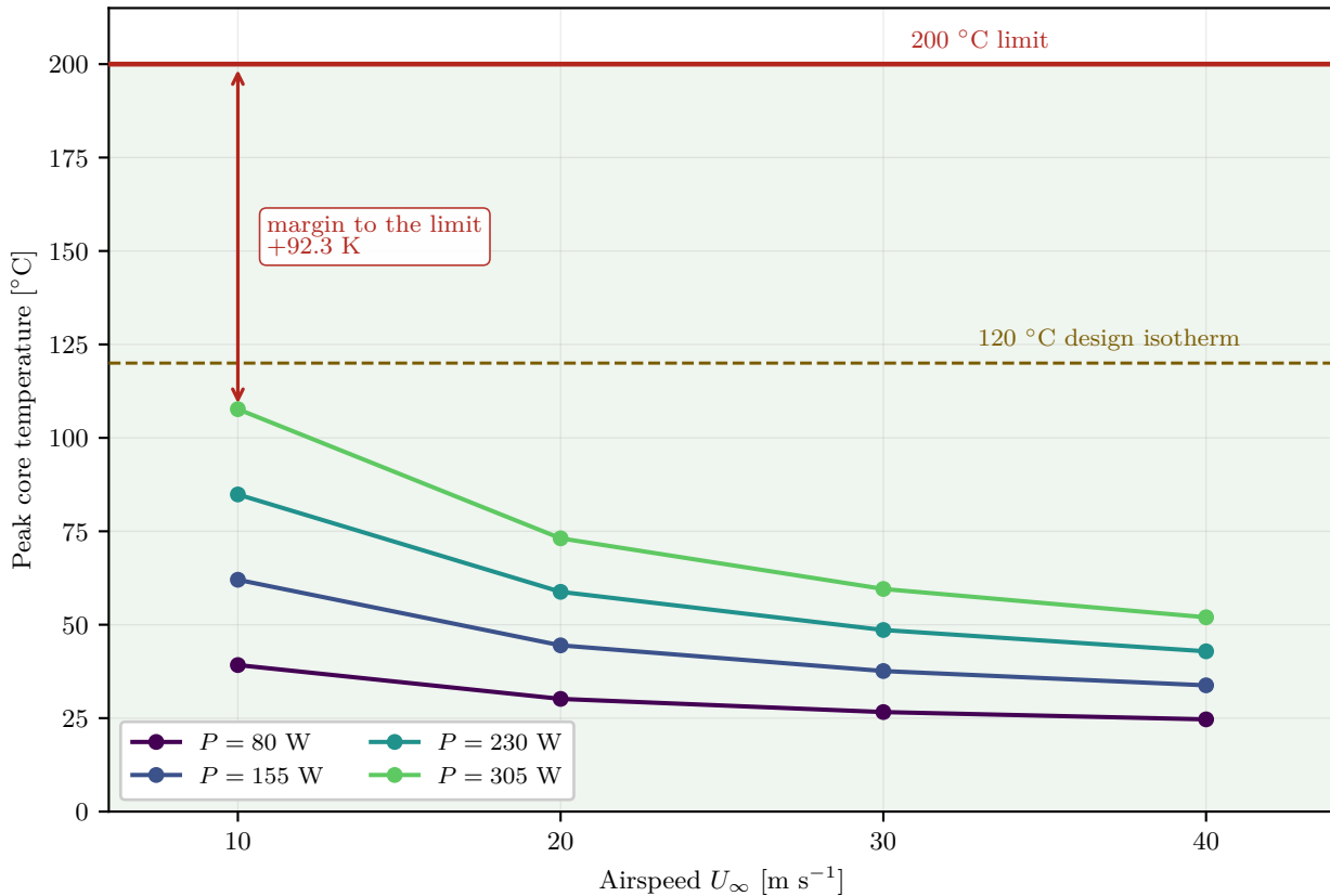
Peak core temperature against airspeed
