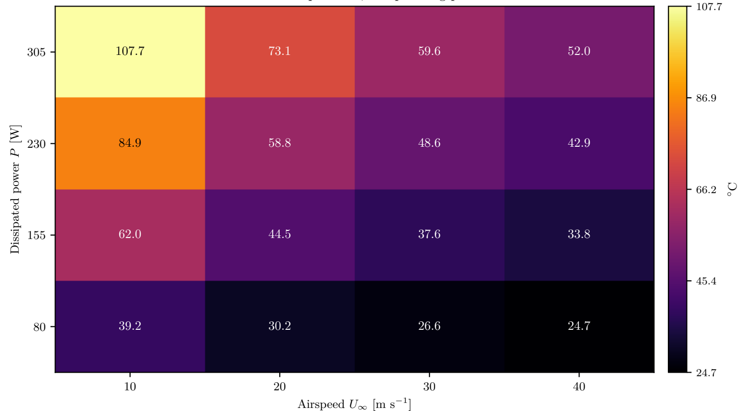
Peak core temperature, 16 operating points
