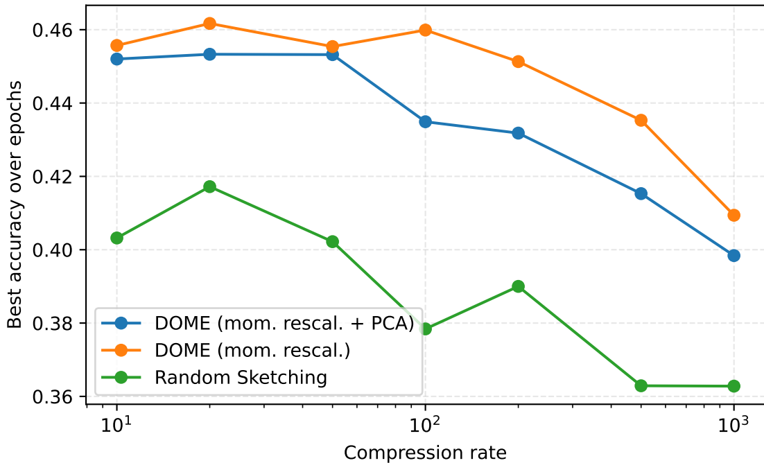
Best accuracy vs compression (dp_scale = 1.0)
