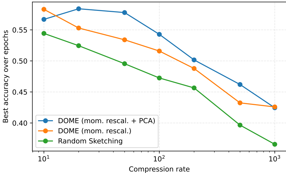
Best accuracy vs compression (dp_scale = 0.2)
