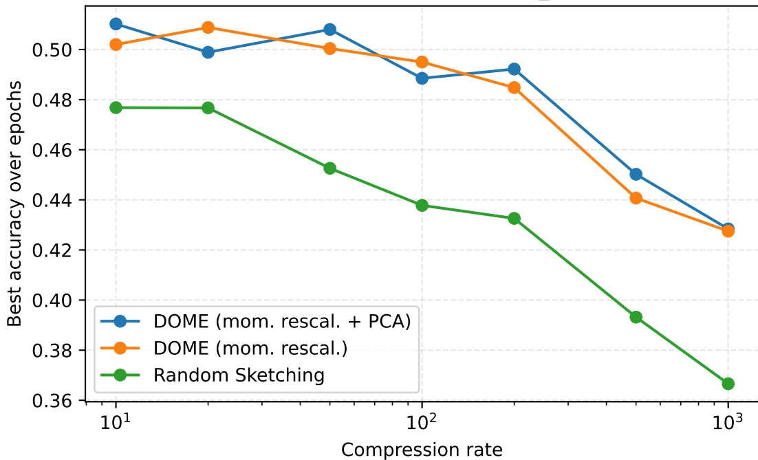
Best accuracy vs compression (dp_scale = 0.5)
