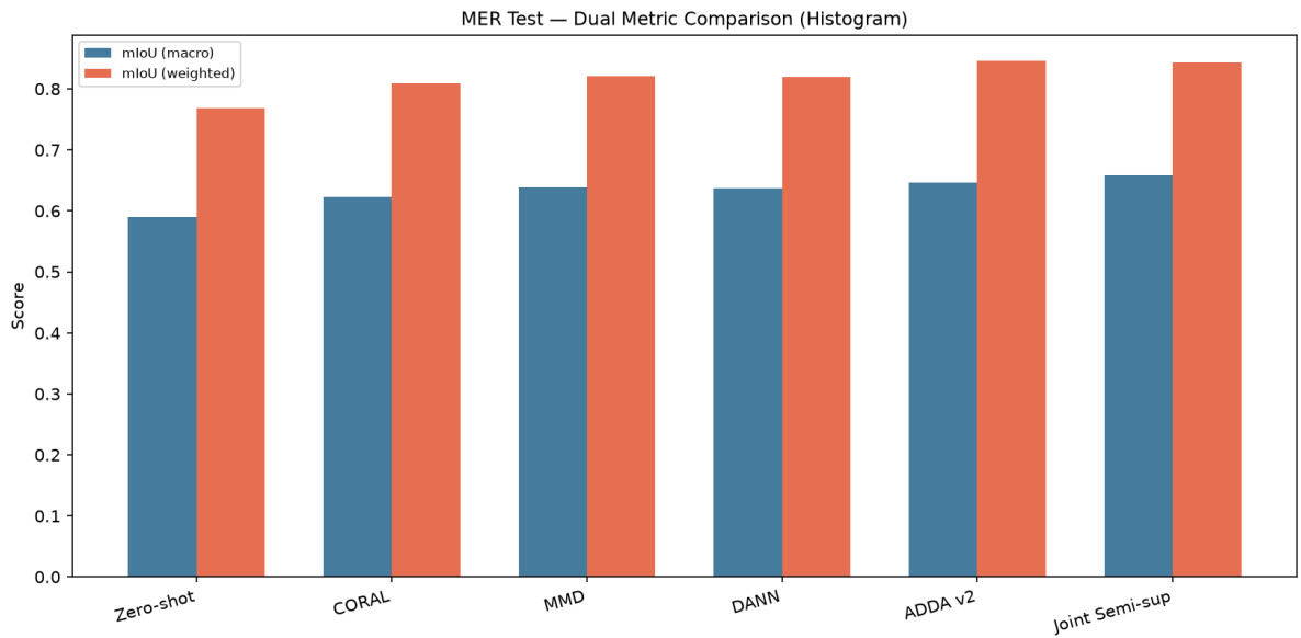
Figure 6: MER test mIoU and wIoU across main-pipeline methods (six key methods).
