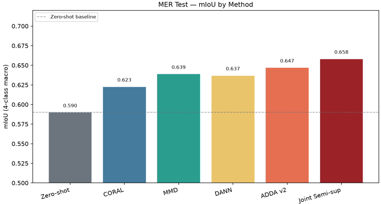
Figure 7: MER test mIoU ranking: zero-shot pretrain, feature UDA methods and joint semi-supervision.
