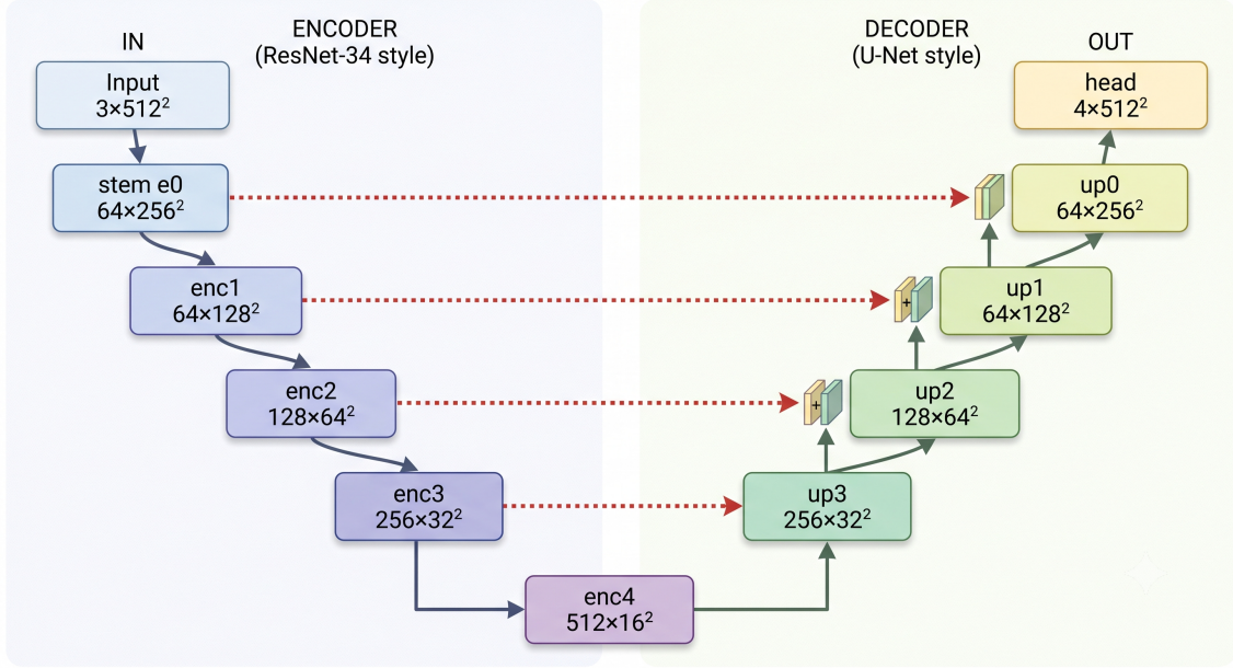
Figure 4: ResNet34-U-Net architecture: ImageNet-pretrained encoder, skip connections at four scales, bottleneck enc4 ( 512 \times 16 \times 16 ) for feature-level UDA and decoder head producing 512 \times 512 class logits.
