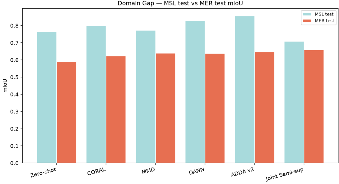
Figure 3: Domain gap: MSL test vs. MER test mIoU (zero-shot pretrain drops \sim 0.17 on MER).
