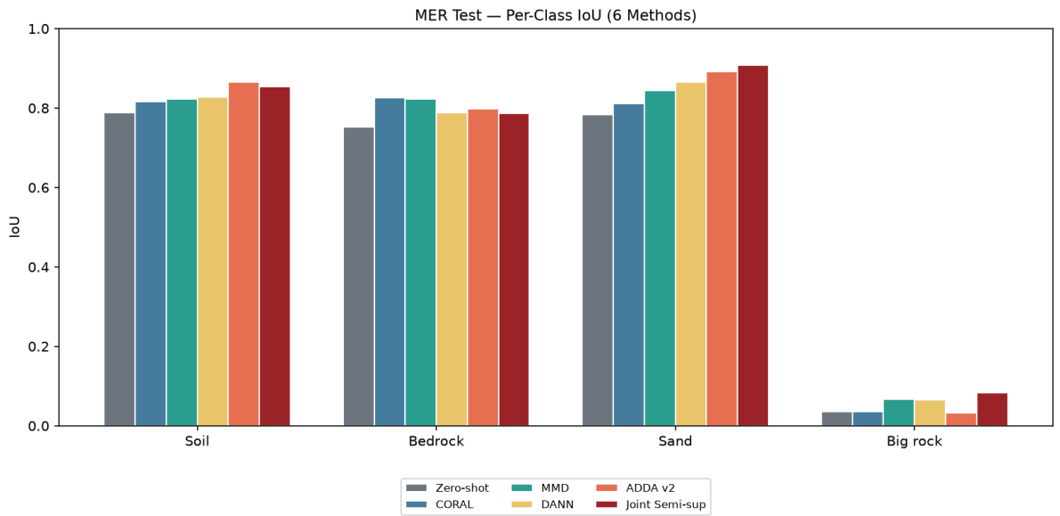
Figure 10: Per-class IoU on MER test across methods (grouped bars).
