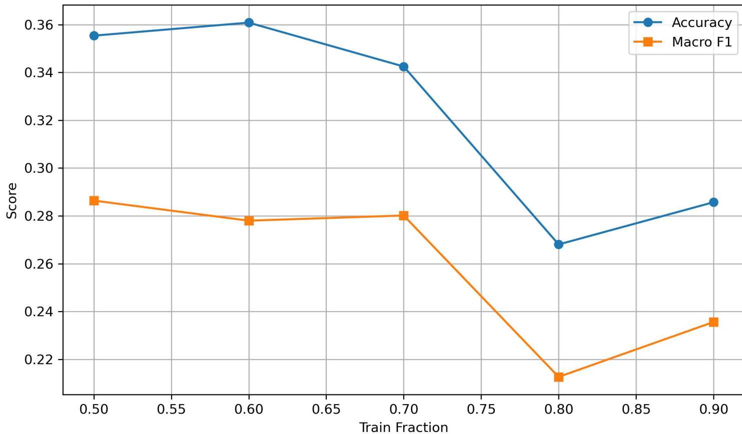
BiLSTM Performance vs Train Fraction
