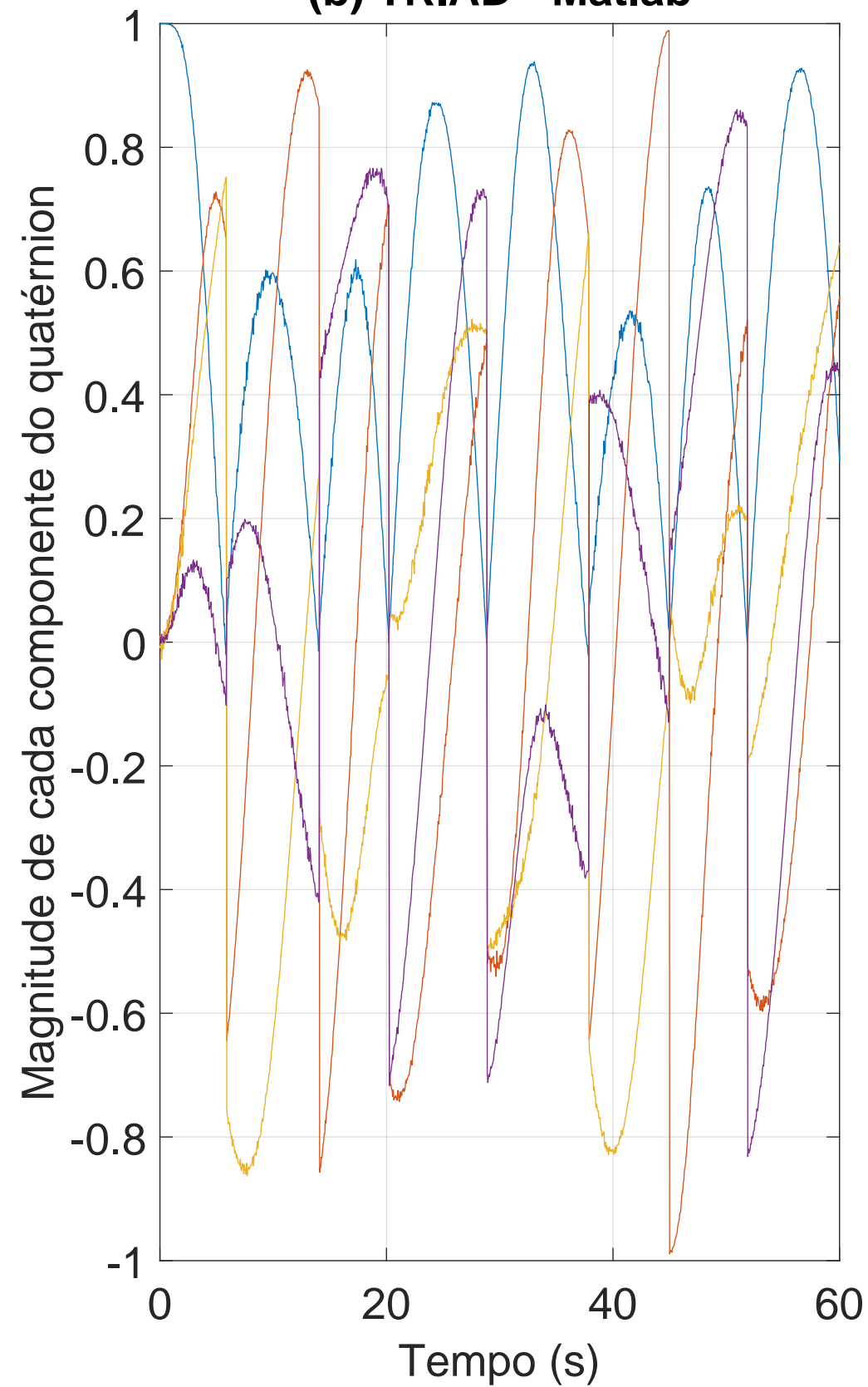
(b) TRIAD - Matlab
