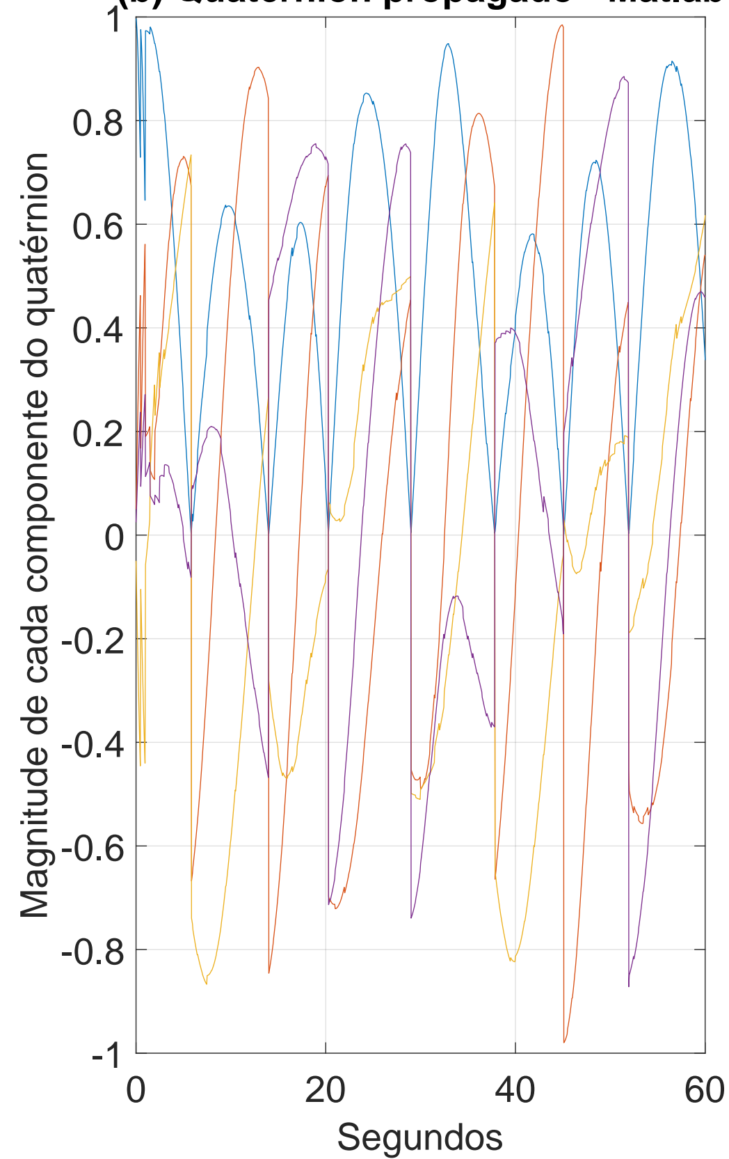
(b) Quatérnion propagado - Matlab
