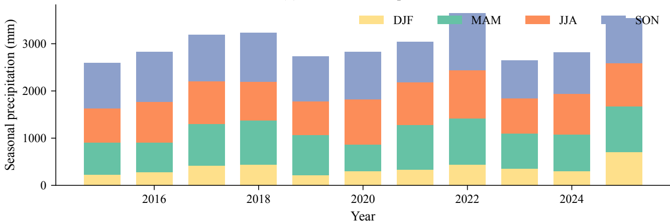
(b) Seasonal decomposition
