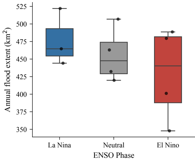
(b) Flood extent by ENSO phase
