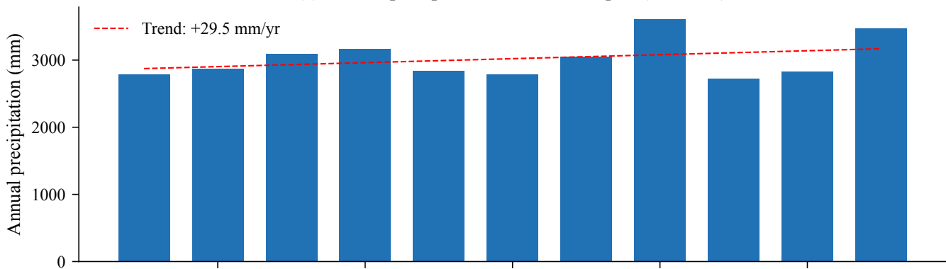
(a) Annual precipitation trend, Antioquia (CHIRPS)
