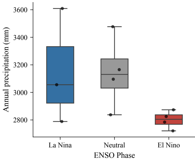
(a) Precipitation by ENSO phase
